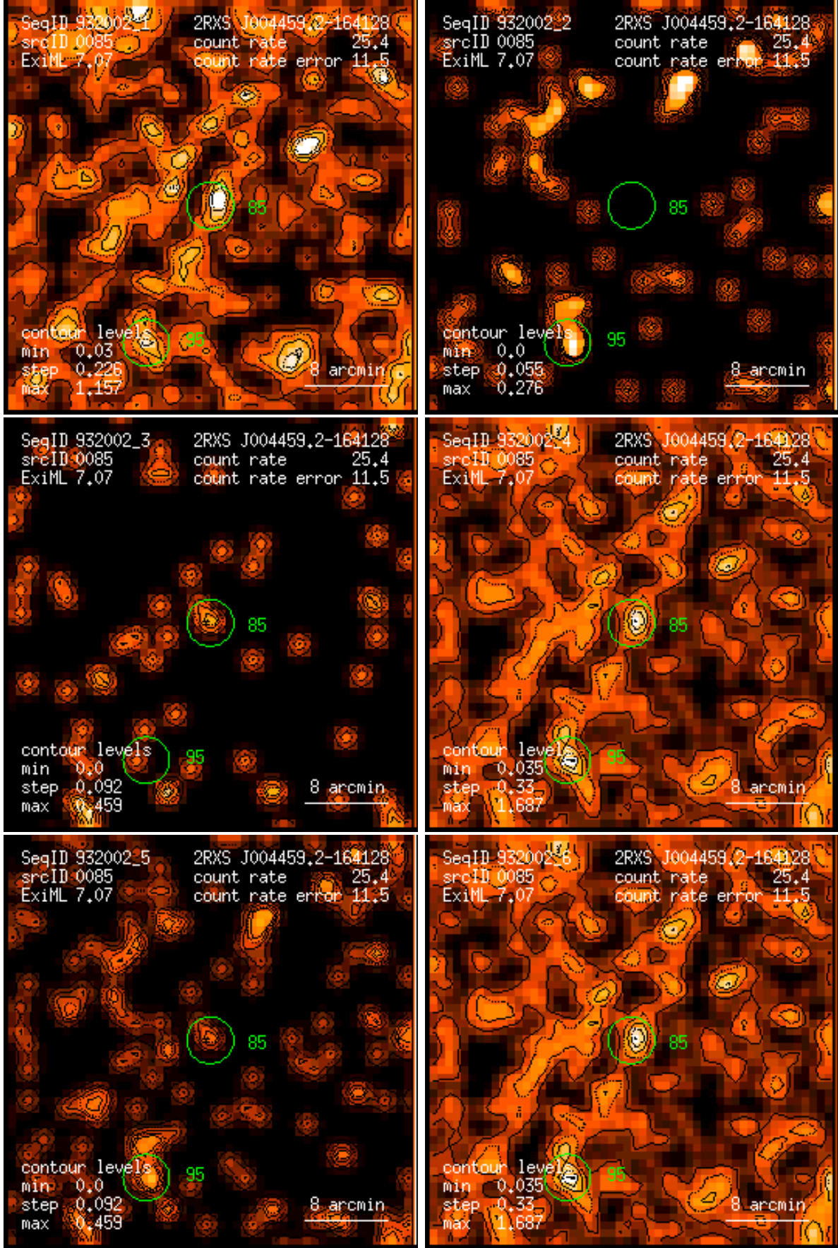
Figure 85: RASS 932002: detection 0085: band rate images, Gaussian filter: (1) PSPC channels 11 – 41, (2) 52 – 90, (3) 91 – 201, (4) 11 – 235, (5) 52 – 201, (6) 11 – 201. Broad band rates in counts/ks. Band rate contour levels in counts/ks/arcmin 2 .
