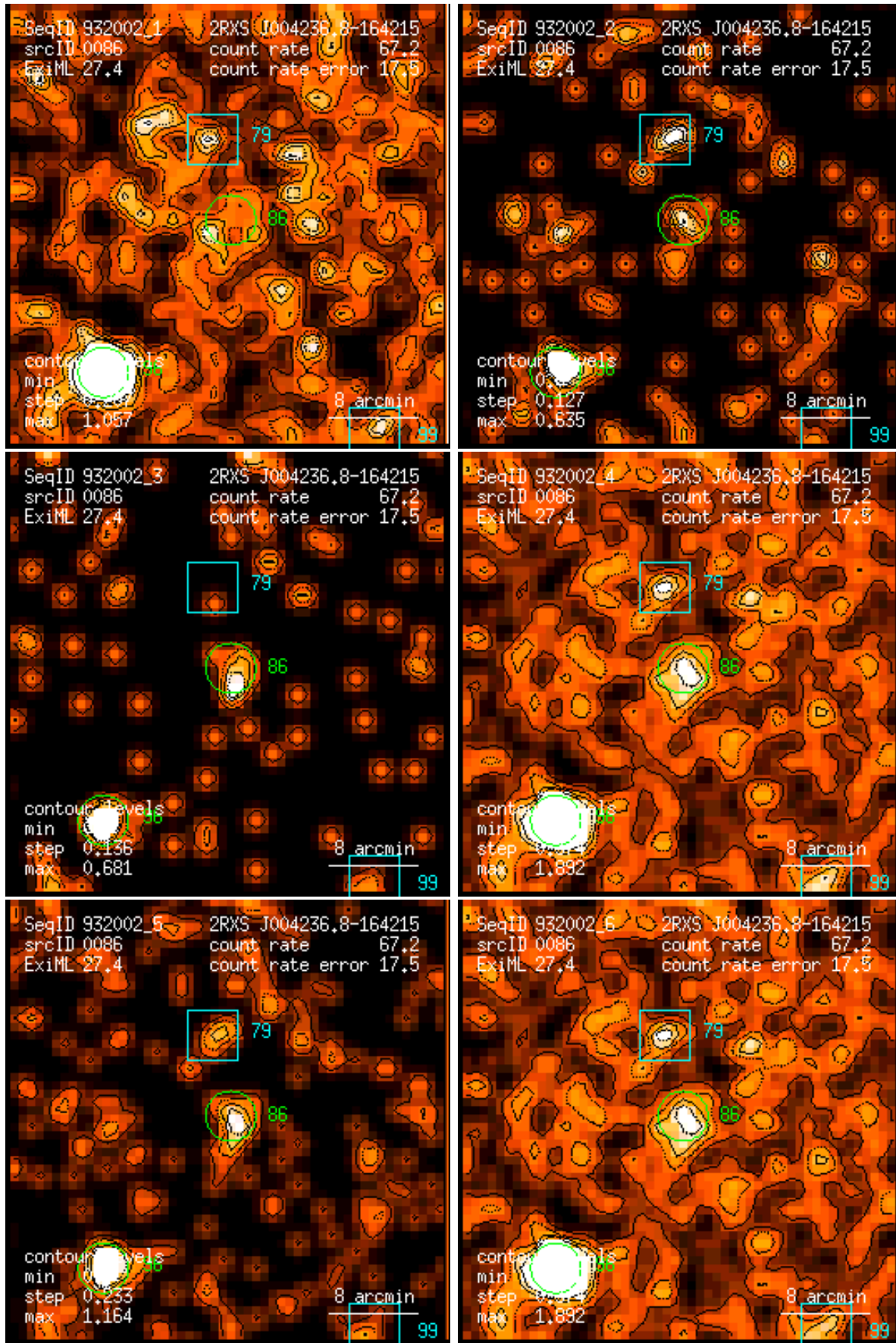
Figure 86: RASS 932002: detection 0086: band rate images, Gaussian filter: (1) PSPC channels 11 – 41, (2) 52 – 90, (3) 91 – 201, (4) 11 – 235, (5) 52 – 201, (6) 11 – 201. Broad band rates in counts/ks. Band rate contour levels in counts/ks/arcmin 2 .
