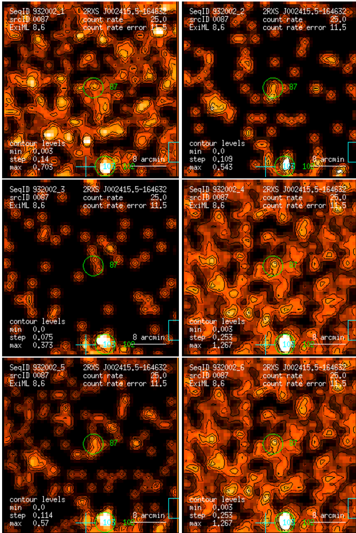
Figure 87: RASS 932002: detection 0087: band rate images, Gaussian filter: (1) PSPC channels 11 – 41, (2) 52 – 90, (3) 91 – 201, (4) 11 – 235, (5) 52 – 201, (6) 11 – 201. Broad band rates in counts/ks. Band rate contour levels in counts/ks/arcmin 2 .
