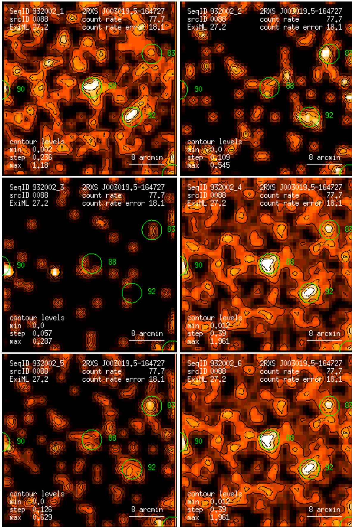
Figure 88: RASS 932002: detection 0088: band rate images, Gaussian filter: (1) PSPC channels 11 – 41, (2) 52 – 90, (3) 91 – 201, (4) 11 – 235, (5) 52 – 201, (6) 11 – 201. Broad band rates in counts/ks. Band rate contour levels in counts/ks/arcmin 2 .
