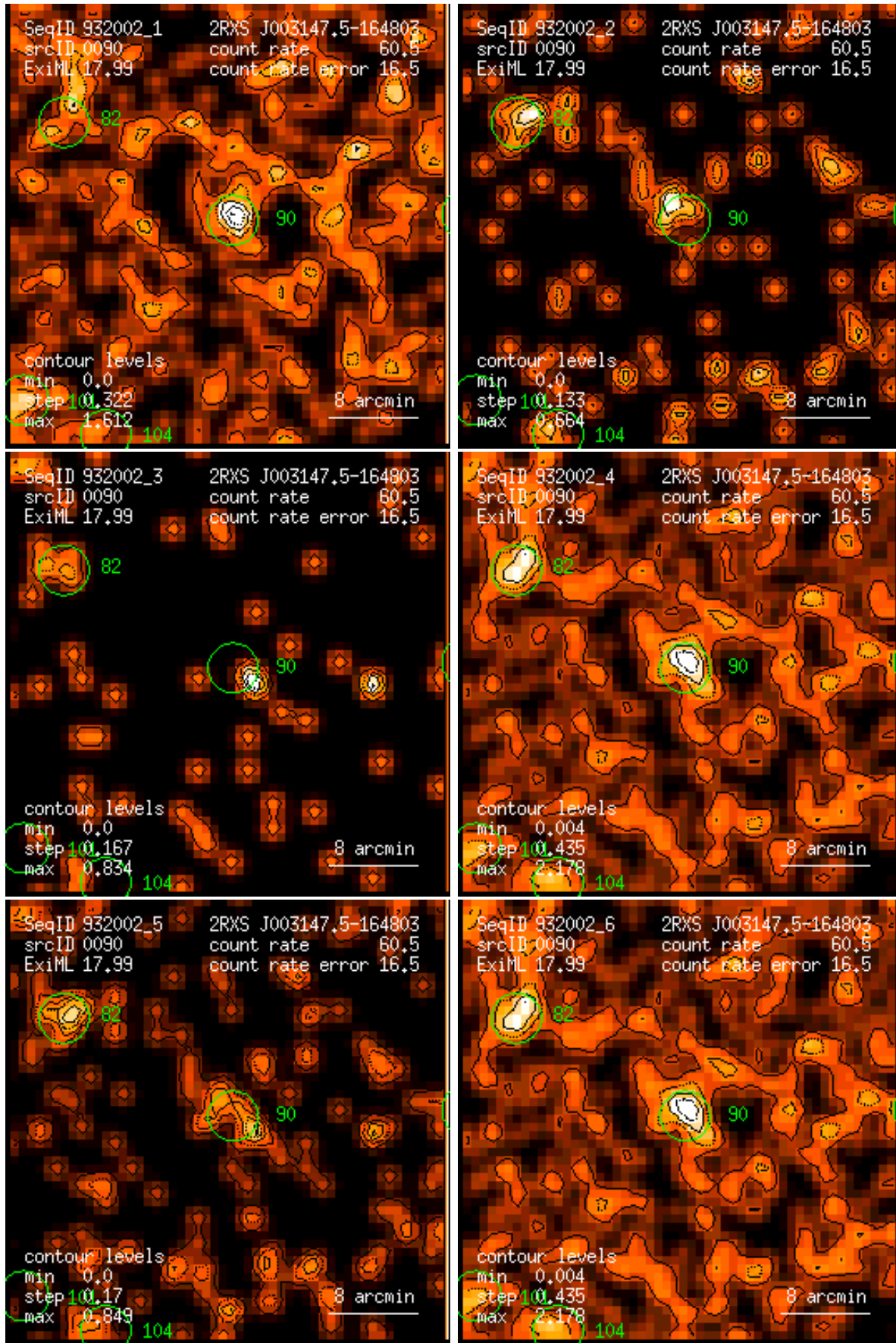
Figure 90: RASS 932002: detection 0090: band rate images, Gaussian filter: (1) PSPC channels 11 – 41, (2) 52 – 90, (3) 91 – 201, (4) 11 – 235, (5) 52 – 201, (6) 11 – 201. Broad band rates in counts/ks. Band rate contour levels in counts/ks/arcmin 2 .
