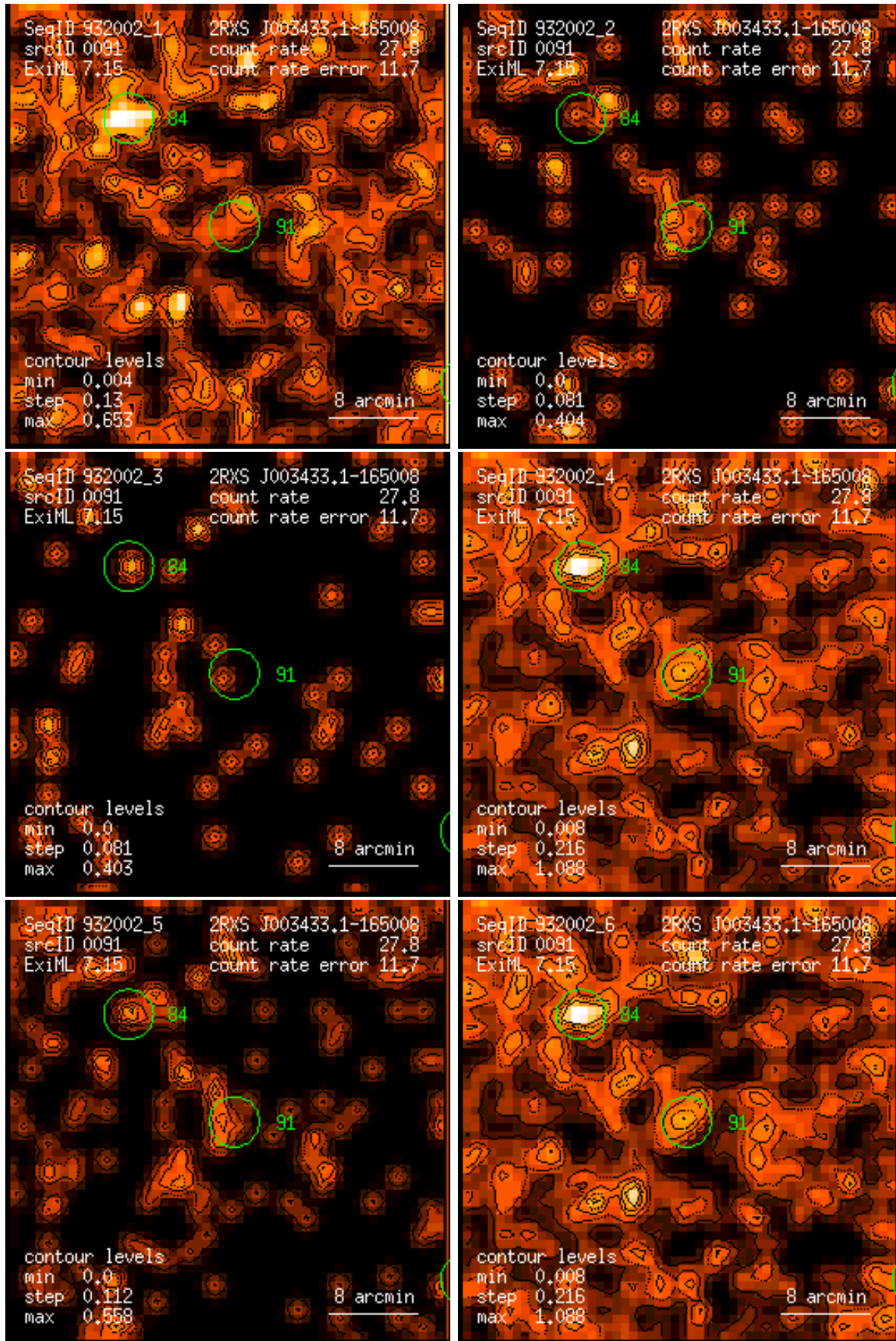
Figure 91: RASS 932002: detection 0091: band rate images, Gaussian filter: (1) PSPC channels 11 – 41, (2) 52 – 90, (3) 91 – 201, (4) 11 – 235, (5) 52 – 201, (6) 11 – 201. Broad band rates in counts/ks. Band rate contour levels in counts/ks/arcmin 2 .
