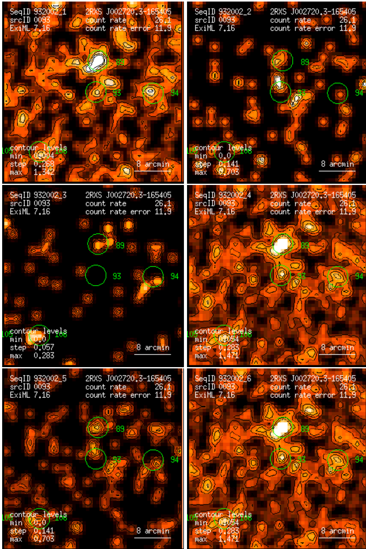
Figure 93: RASS 932002: detection 0093: band rate images, Gaussian filter: (1) PSPC channels 11 – 41, (2) 52 – 90, (3) 91 – 201, (4) 11 – 235, (5) 52 – 201, (6) 11 – 201. Broad band rates in counts/ks. Band rate contour levels in counts/ks/arcmin 2 .
