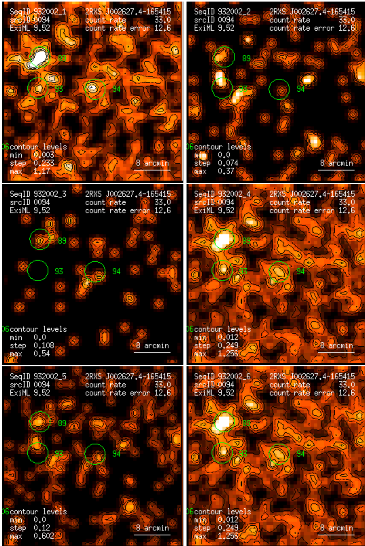
Figure 94: RASS 932002: detection 0094: band rate images, Gaussian filter: (1) PSPC channels 11 – 41, (2) 52 – 90, (3) 91 – 201, (4) 11 – 235, (5) 52 – 201, (6) 11 – 201. Broad band rates in counts/ks. Band rate contour levels in counts/ks/arcmin 2 .
