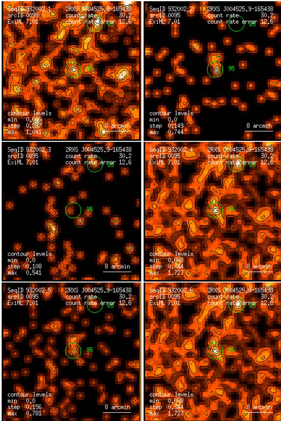
Figure 95: RASS 932002: detection 0095: band rate images, Gaussian filter: (1) PSPC channels 11 – 41, (2) 52 – 90, (3) 91 – 201, (4) 11 – 235, (5) 52 – 201, (6) 11 – 201. Broad band rates in counts/ks. Band rate contour levels in counts/ks/arcmin 2 .
