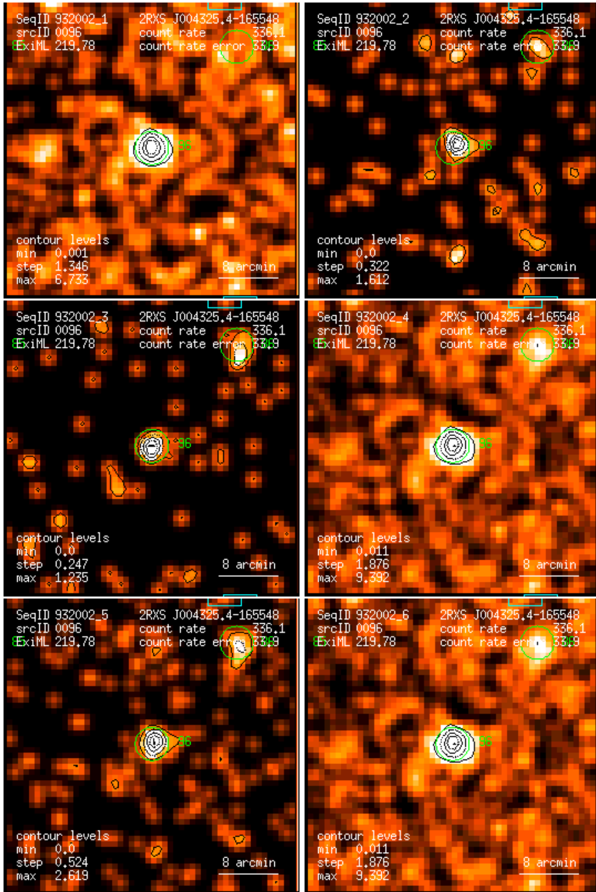
Figure 96: RASS 932002: detection 0096: band rate images, Gaussian filter: (1) PSPC channels 11 – 41, (2) 52 – 90, (3) 91 – 201, (4) 11 – 235, (5) 52 – 201, (6) 11 – 201. Broad band rates in counts/ks. Band rate contour levels in counts/ks/arcmin 2 .
