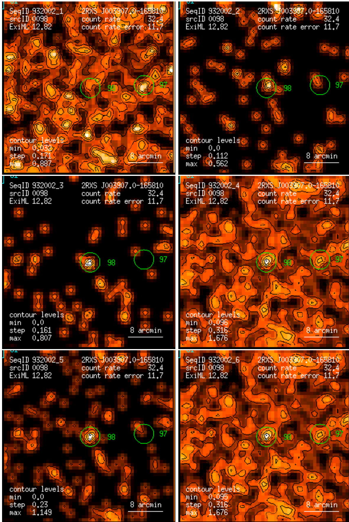
Figure 98: RASS 932002: detection 0098: band rate images, Gaussian filter: (1) PSPC channels 11 – 41, (2) 52 – 90, (3) 91 – 201, (4) 11 – 235, (5) 52 – 201, (6) 11 – 201. Broad band rates in counts/ks. Band rate contour levels in counts/ks/arcmin 2 .
