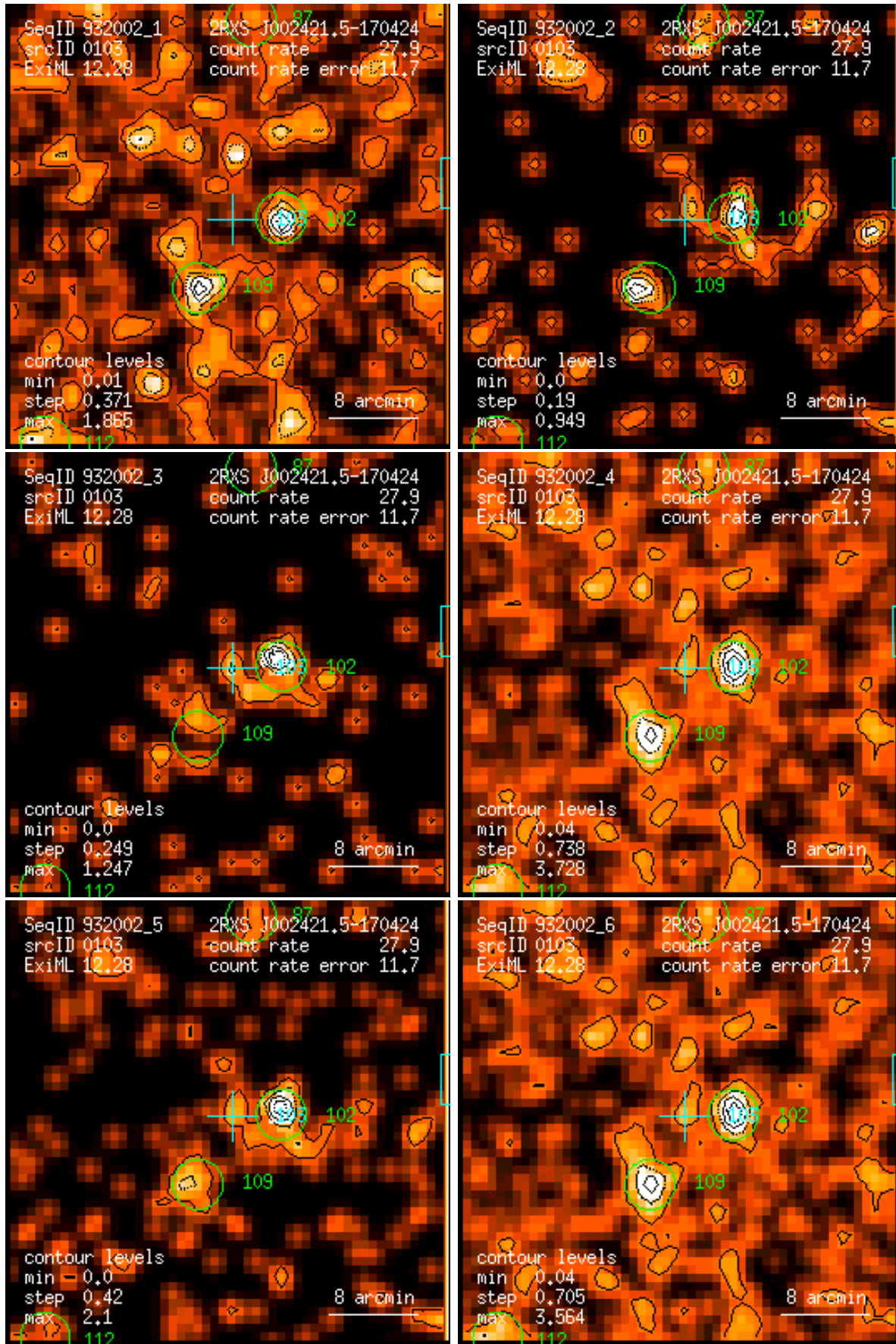
Figure 103: RASS 932002: detection 0103: band rate images, Gaussian filter: (1) PSPC channels 11 – 41, (2) 52 – 90, (3) 91 – 201, (4) 11 – 235, (5) 52 – 201, (6) 11 – 201. Broad band rates in counts/ks. Band rate contour levels in counts/ks/arcmin 2 .
