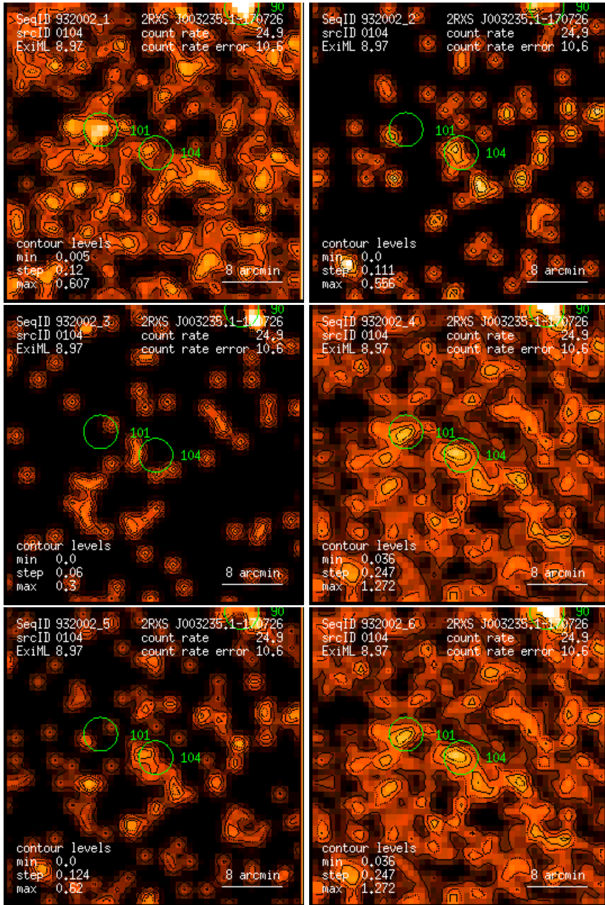
Figure 104: RASS 932002: detection 0104: band rate images, Gaussian filter: (1) PSPC channels 11 – 41, (2) 52 – 90, (3) 91 – 201, (4) 11 – 235, (5) 52 – 201, (6) 11 – 201. Broad band rates in counts/ks. Band rate contour levels in counts/ks/arcmin 2 .
