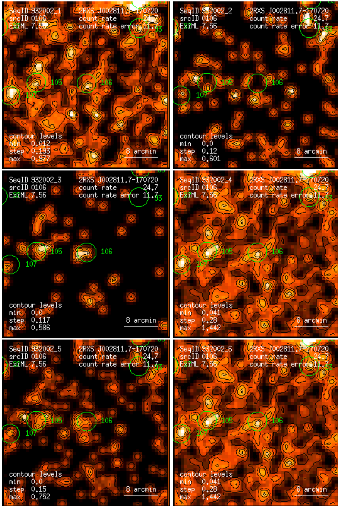
Figure 106: RASS 932002: detection 0106: band rate images, Gaussian filter: (1) PSPC channels 11 – 41, (2) 52 – 90, (3) 91 – 201, (4) 11 – 235, (5) 52 – 201, (6) 11 – 201. Broad band rates in counts/ks. Band rate contour levels in counts/ks/arcmin 2 .
