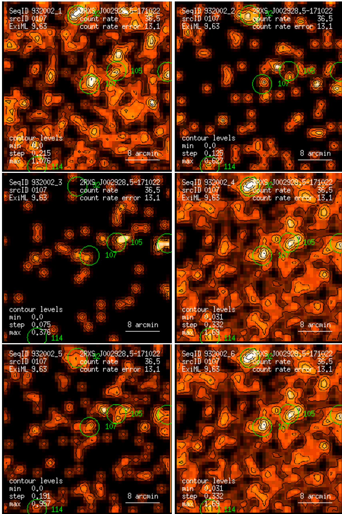
Figure 107: RASS 932002: detection 0107: band rate images, Gaussian filter: (1) PSPC channels 11 – 41, (2) 52 – 90, (3) 91 – 201, (4) 11 – 235, (5) 52 – 201, (6) 11 – 201. Broad band rates in counts/ks. Band rate contour levels in counts/ks/arcmin 2 .
