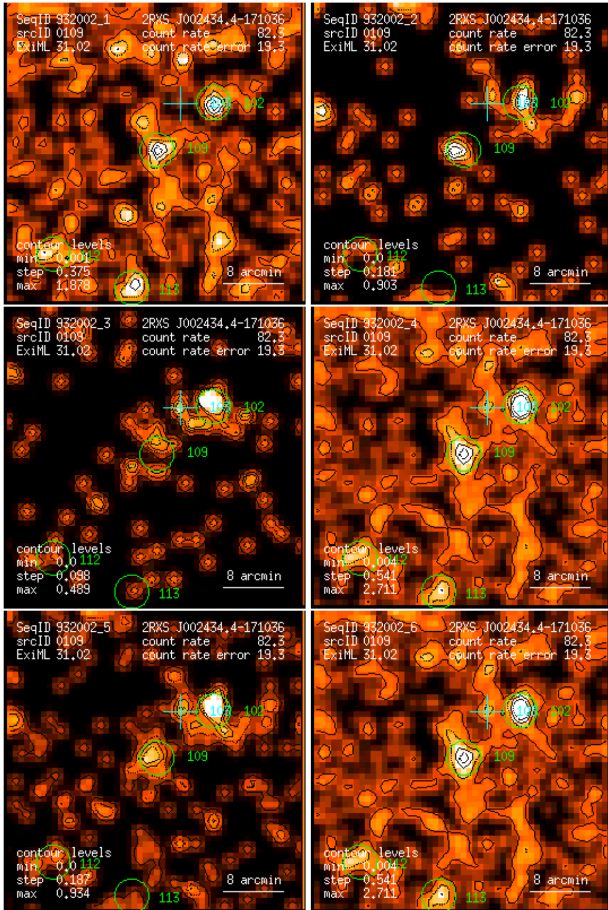
Figure 109: RASS 932002: detection 0109: band rate images, Gaussian filter: (1) PSPC channels 11 – 41, (2) 52 – 90, (3) 91 – 201, (4) 11 – 235, (5) 52 – 201, (6) 11 – 201. Broad band rates in counts/ks. Band rate contour levels in counts/ks/arcmin 2 .
