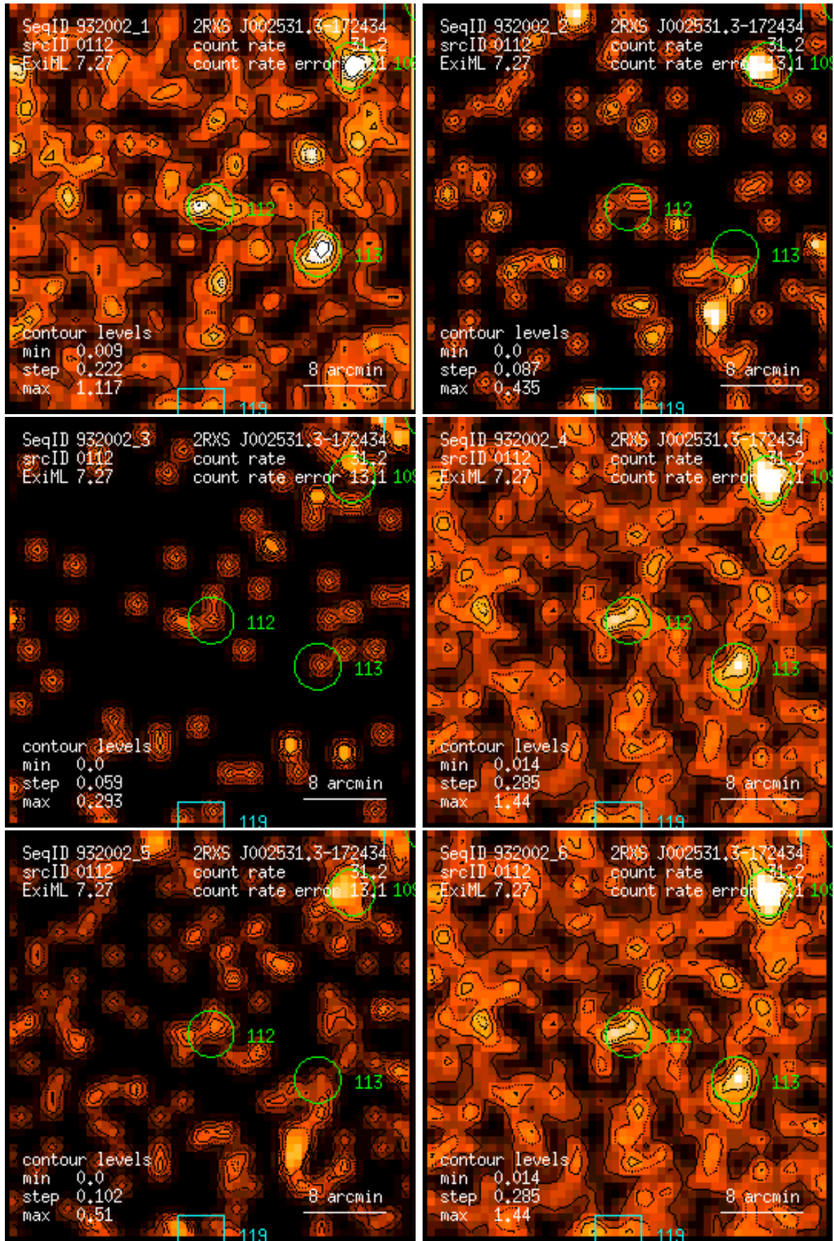
Figure 112: RASS 932002: detection 0112: band rate images, Gaussian filter: (1) PSPC channels 11 – 41, (2) 52 – 90, (3) 91 – 201, (4) 11 – 235, (5) 52 – 201, (6) 11 – 201. Broad band rates in counts/ks. Band rate contour levels in counts/ks/arcmin 2 .
