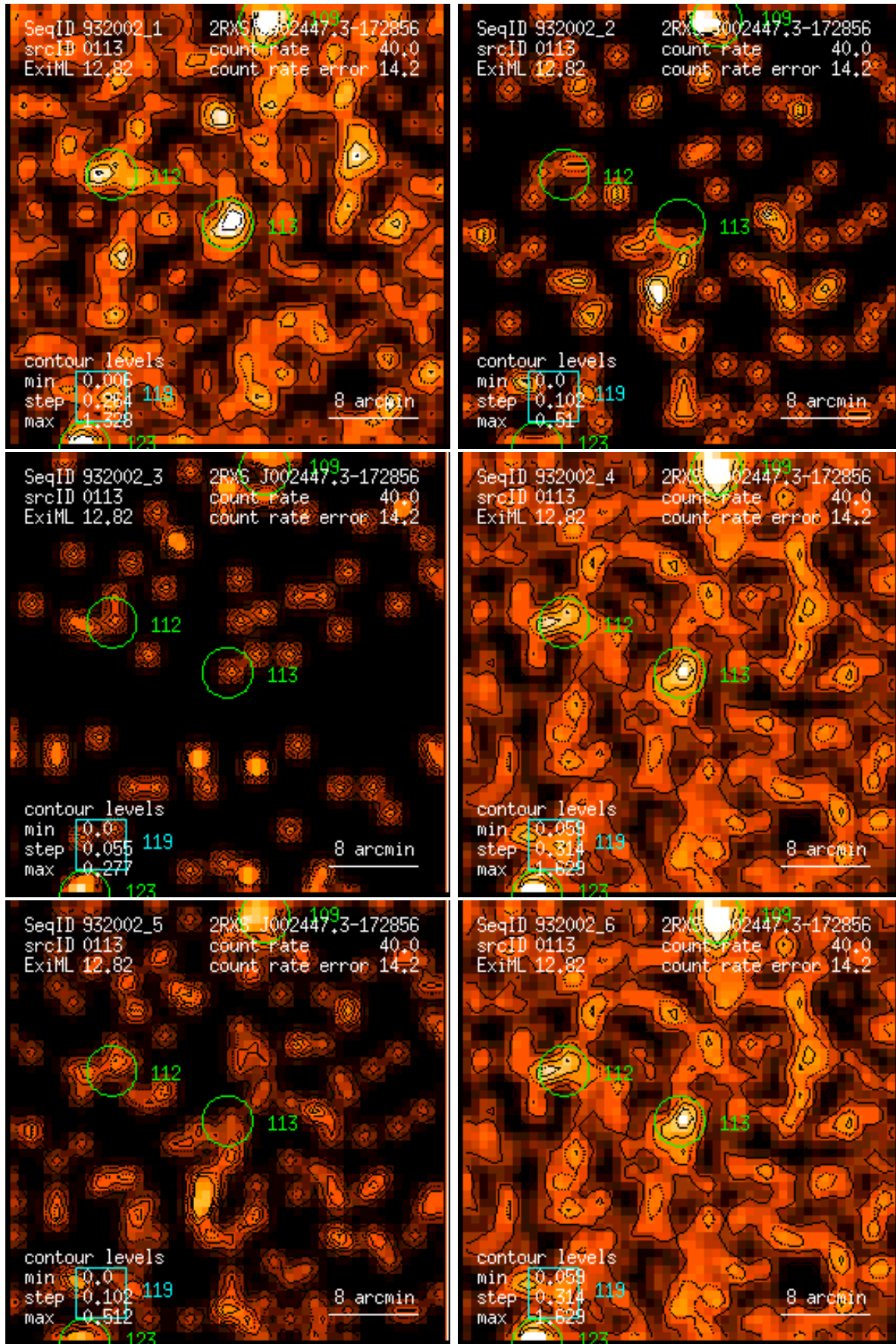
Figure 113: RASS 932002: detection 0113: band rate images, Gaussian filter: (1) PSPC channels 11 – 41, (2) 52 – 90, (3) 91 – 201, (4) 11 – 235, (5) 52 – 201, (6) 11 – 201. Broad band rates in counts/ks. Band rate contour levels in counts/ks/arcmin 2 .
