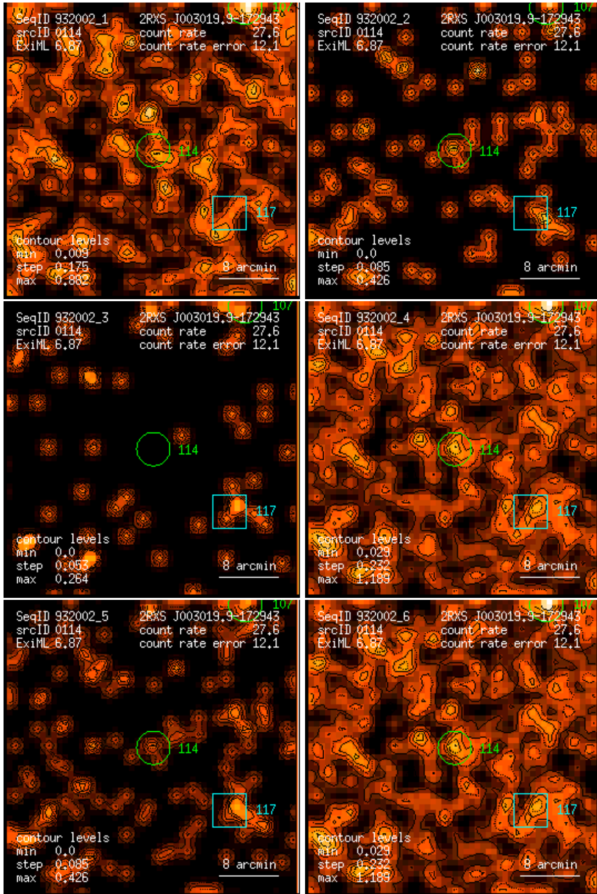
Figure 114: RASS 932002: detection 0114: band rate images, Gaussian filter: (1) PSPC channels 11 – 41, (2) 52 – 90, (3) 91 – 201, (4) 11 – 235, (5) 52 – 201, (6) 11 – 201. Broad band rates in counts/ks. Band rate contour levels in counts/ks/arcmin 2 .
