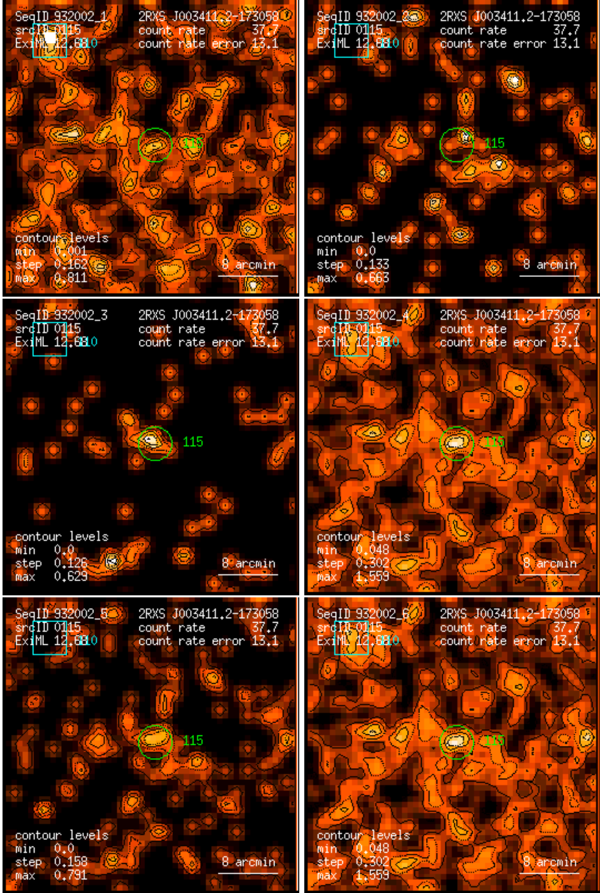
Figure 115: RASS 932002: detection 0115: band rate images, Gaussian filter: (1) PSPC channels 11 – 41, (2) 52 – 90, (3) 91 – 201, (4) 11 – 235, (5) 52 – 201, (6) 11 – 201. Broad band rates in counts/ks. Band rate contour levels in counts/ks/arcmin 2 .
