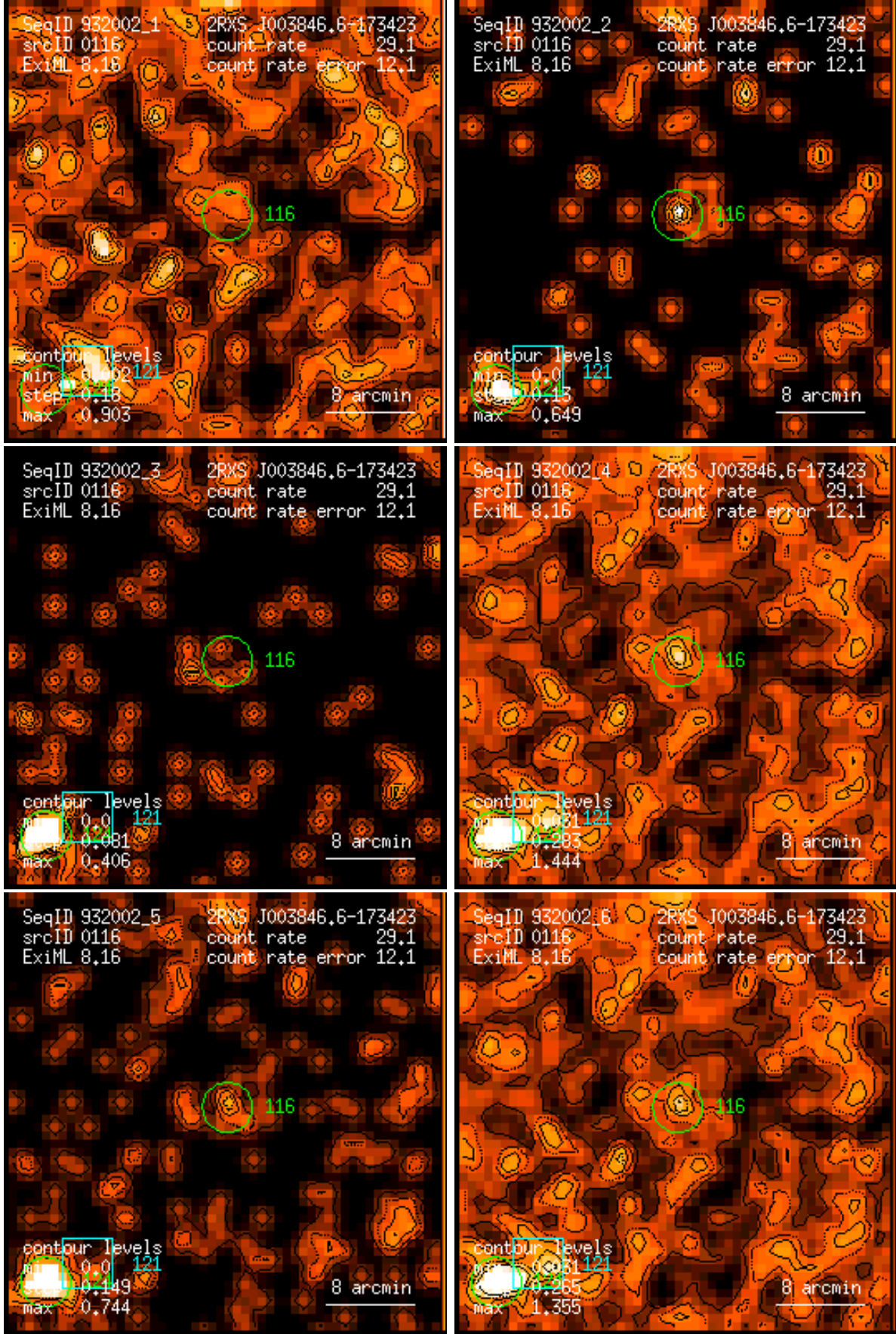
Figure 116: RASS 932002: detection 0116: band rate images, Gaussian filter: (1) PSPC channels 11 – 41, (2) 52 – 90, (3) 91 – 201, (4) 11 – 235, (5) 52 – 201, (6) 11 – 201. Broad band rates in counts/ks. Band rate contour levels in counts/ks/arcmin 2 .
