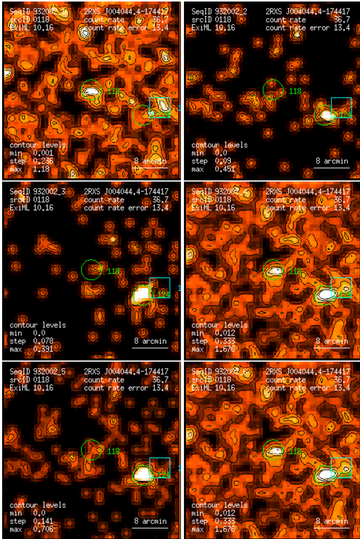
Figure 118: RASS 932002: detection 0118: band rate images, Gaussian filter: (1) PSPC channels 11 – 41, (2) 52 – 90, (3) 91 – 201, (4) 11 – 235, (5) 52 – 201, (6) 11 – 201. Broad band rates in counts/ks. Band rate contour levels in counts/ks/arcmin 2 .
