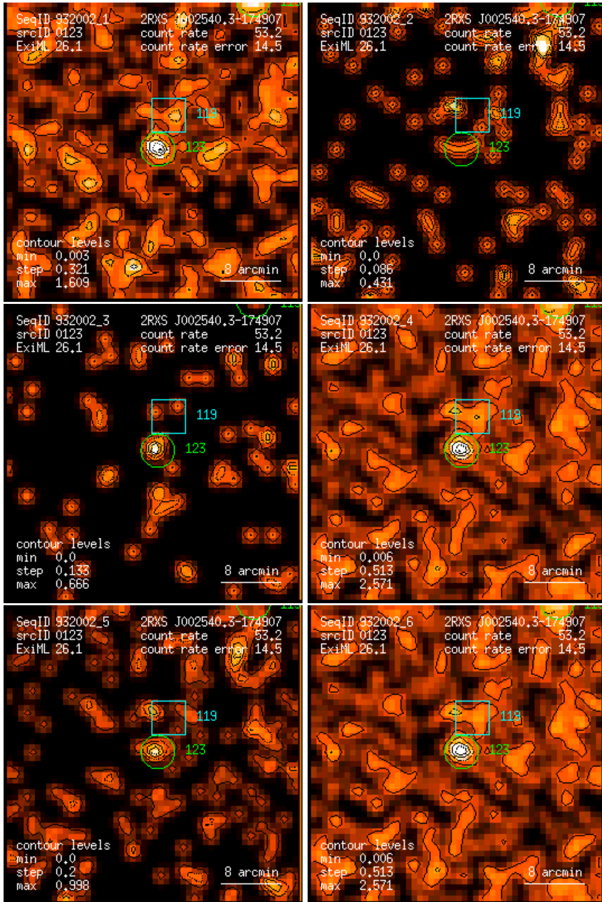
Figure 123: RASS 932002: detection 0123: band rate images, Gaussian filter: (1) PSPC channels 11 – 41, (2) 52 – 90, (3) 91 – 201, (4) 11 – 235, (5) 52 – 201, (6) 11 – 201. Broad band rates in counts/ks. Band rate contour levels in counts/ks/arcmin 2 .
