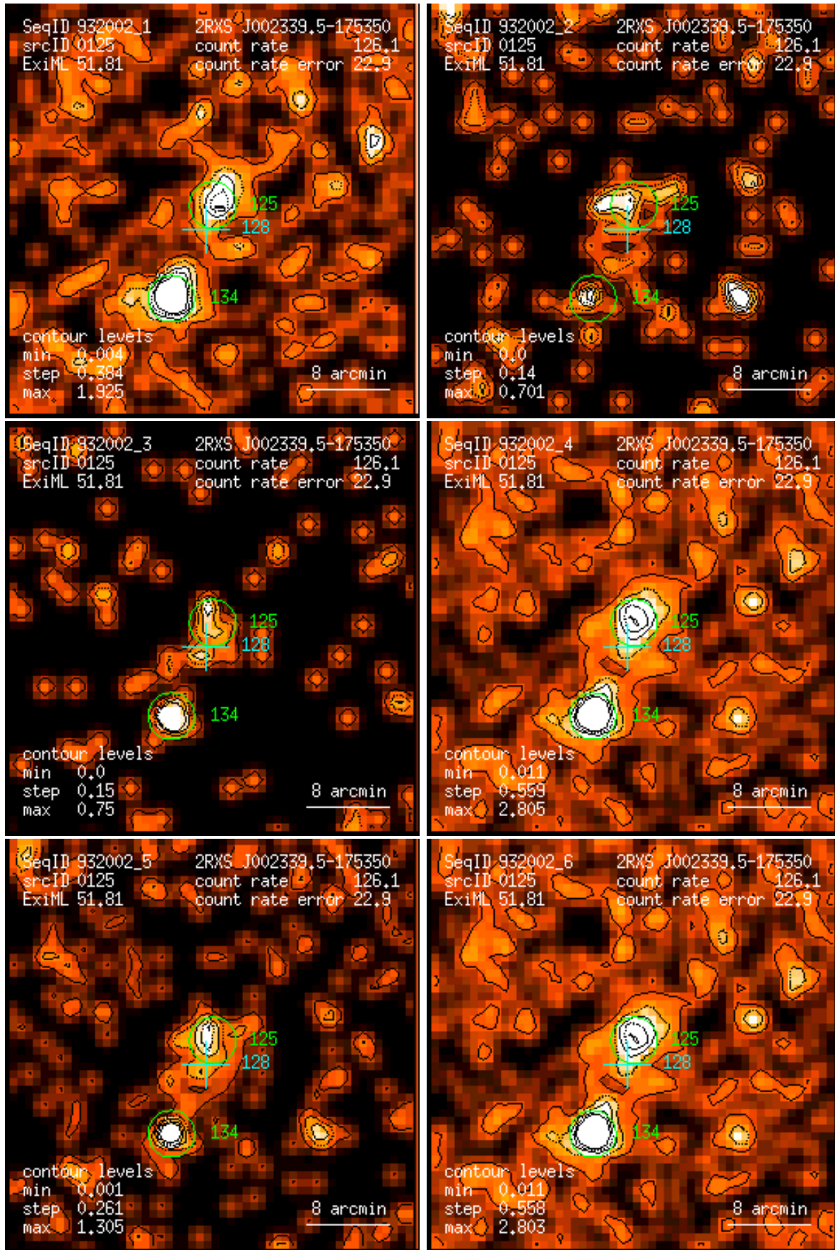
Figure 125: RASS 932002: detection 0125: band rate images, Gaussian filter: (1) PSPC channels 11 – 41, (2) 52 – 90, (3) 91 – 201, (4) 11 – 235, (5) 52 – 201, (6) 11 – 201. Broad band rates in counts/ks. Band rate contour levels in counts/ks/arcmin 2 .
