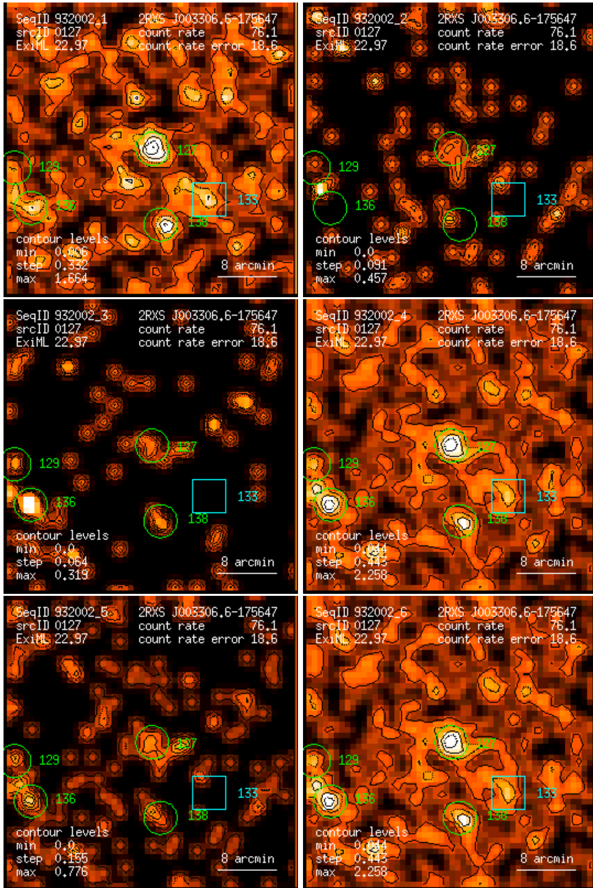
Figure 127: RASS 932002: detection 0127: band rate images, Gaussian filter: (1) PSPC channels 11 – 41, (2) 52 – 90, (3) 91 – 201, (4) 11 – 235, (5) 52 – 201, (6) 11 – 201. Broad band rates in counts/ks. Band rate contour levels in counts/ks/arcmin 2 .
