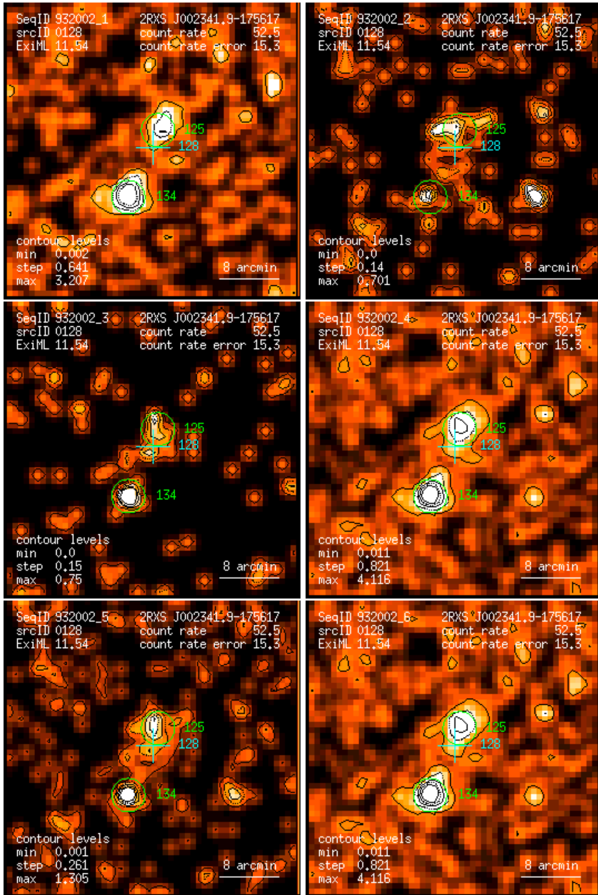
Figure 128: RASS 932002: detection 0128: band rate images, Gaussian filter: (1) PSPC channels 11 – 41, (2) 52 – 90, (3) 91 – 201, (4) 11 – 235, (5) 52 – 201, (6) 11 – 201. Broad band rates in counts/ks. Band rate contour levels in counts/ks/arcmin 2 .
