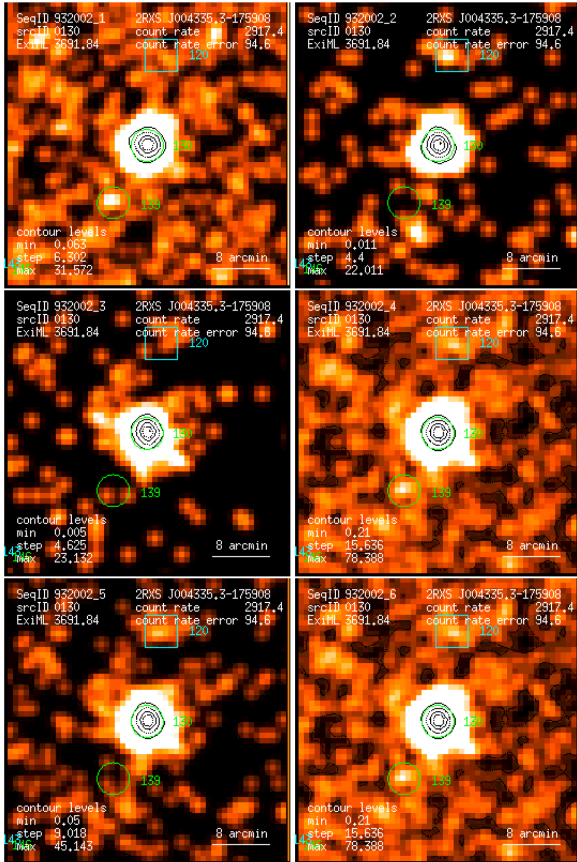
Figure 130: RASS 932002: detection 0130: band rate images, Gaussian filter: (1) PSPC channels 11 – 41, (2) 52 – 90, (3) 91 – 201, (4) 11 – 235, (5) 52 – 201, (6) 11 – 201. Broad band rates in counts/ks. Band rate contour levels in counts/ks/arcmin 2 .
