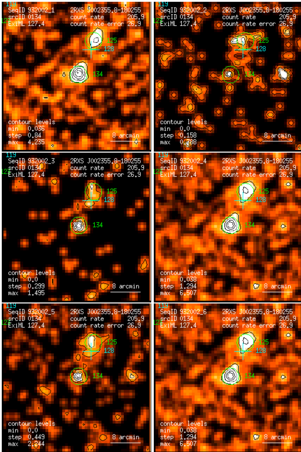
Figure 134: RASS 932002: detection 0134: band rate images, Gaussian filter: (1) PSPC channels 11 – 41, (2) 52 – 90, (3) 91 – 201, (4) 11 – 235, (5) 52 – 201, (6) 11 – 201. Broad band rates in counts/ks. Band rate contour levels in counts/ks/arcmin 2 .
