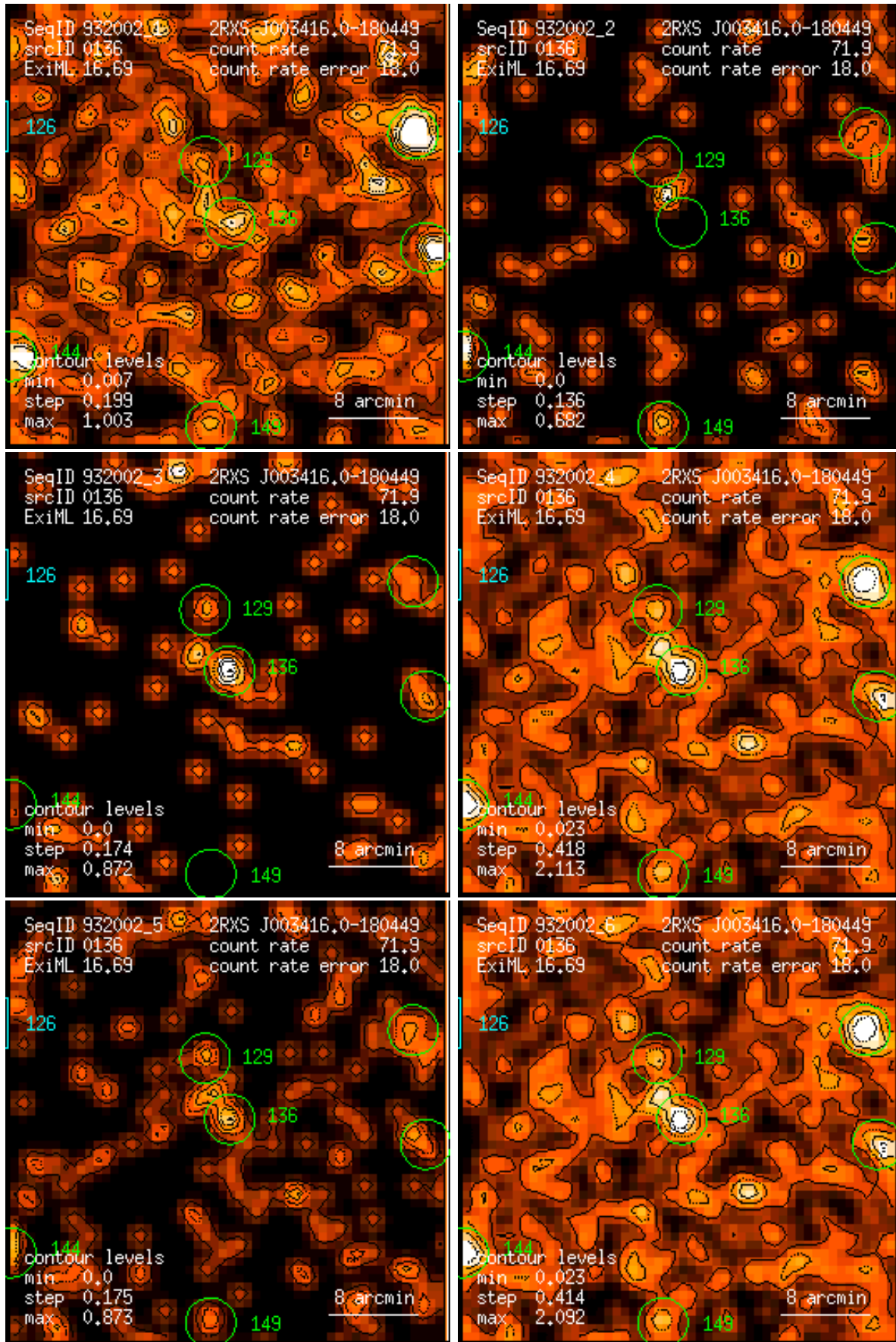
Figure 136: RASS 932002: detection 0136: band rate images, Gaussian filter: (1) PSPC channels 11 – 41, (2) 52 – 90, (3) 91 – 201, (4) 11 – 235, (5) 52 – 201, (6) 11 – 201. Broad band rates in counts/ks. Band rate contour levels in counts/ks/arcmin 2 .
