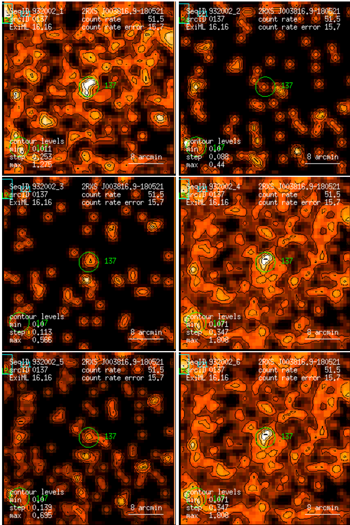
Figure 137: RASS 932002: detection 0137: band rate images, Gaussian filter: (1) PSPC channels 11 – 41, (2) 52 – 90, (3) 91 – 201, (4) 11 – 235, (5) 52 – 201, (6) 11 – 201. Broad band rates in counts/ks. Band rate contour levels in counts/ks/arcmin 2 .
