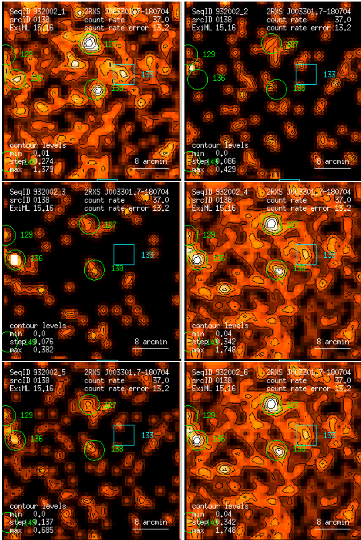
Figure 138: RASS 932002: detection 0138: band rate images, Gaussian filter: (1) PSPC channels 11 – 41, (2) 52 – 90, (3) 91 – 201, (4) 11 – 235, (5) 52 – 201, (6) 11 – 201. Broad band rates in counts/ks. Band rate contour levels in counts/ks/arcmin 2 .
