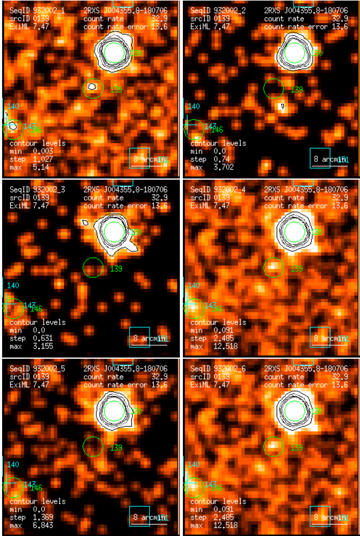
Figure 139: RASS 932002: detection 0139: band rate images, Gaussian filter: (1) PSPC channels 11 – 41, (2) 52 – 90, (3) 91 – 201, (4) 11 – 235, (5) 52 – 201, (6) 11 – 201. Broad band rates in counts/ks. Band rate contour levels in counts/ks/arcmin 2 .
