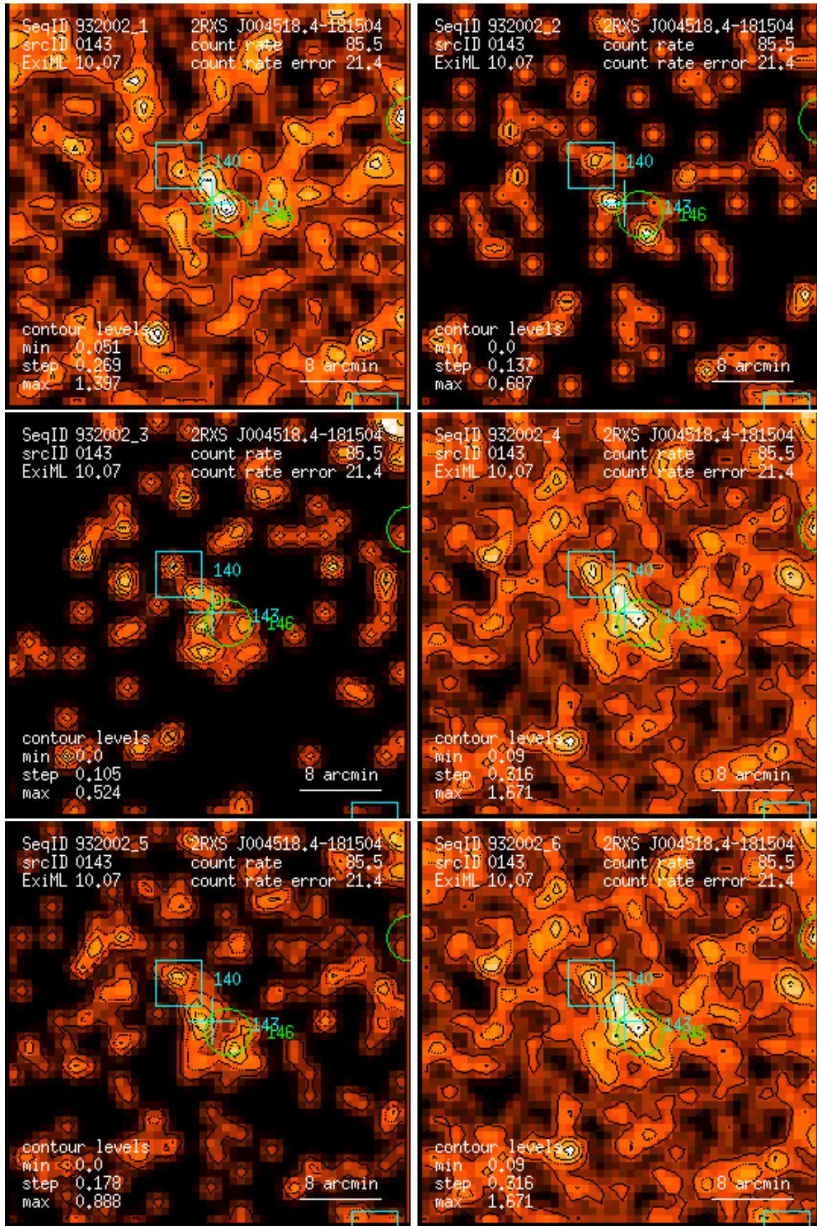
Figure 143: RASS 932002: detection 0143: band rate images, Gaussian filter: (1) PSPC channels 11 – 41, (2) 52 – 90, (3) 91 – 201, (4) 11 – 235, (5) 52 – 201, (6) 11 – 201. Broad band rates in counts/ks. Band rate contour levels in counts/ks/arcmin 2 .
