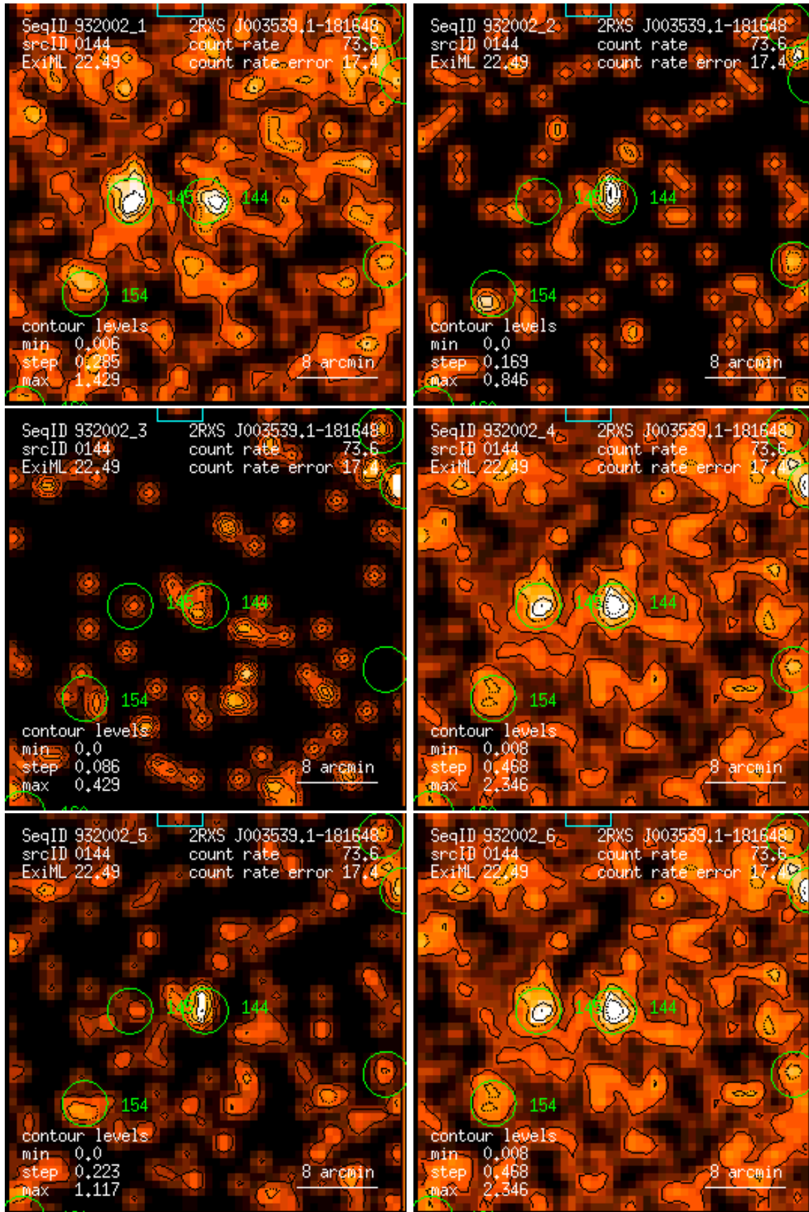
Figure 144: RASS 932002: detection 0144: band rate images, Gaussian filter: (1) PSPC channels 11 – 41, (2) 52 – 90, (3) 91 – 201, (4) 11 – 235, (5) 52 – 201, (6) 11 – 201. Broad band rates in counts/ks. Band rate contour levels in counts/ks/arcmin 2 .
