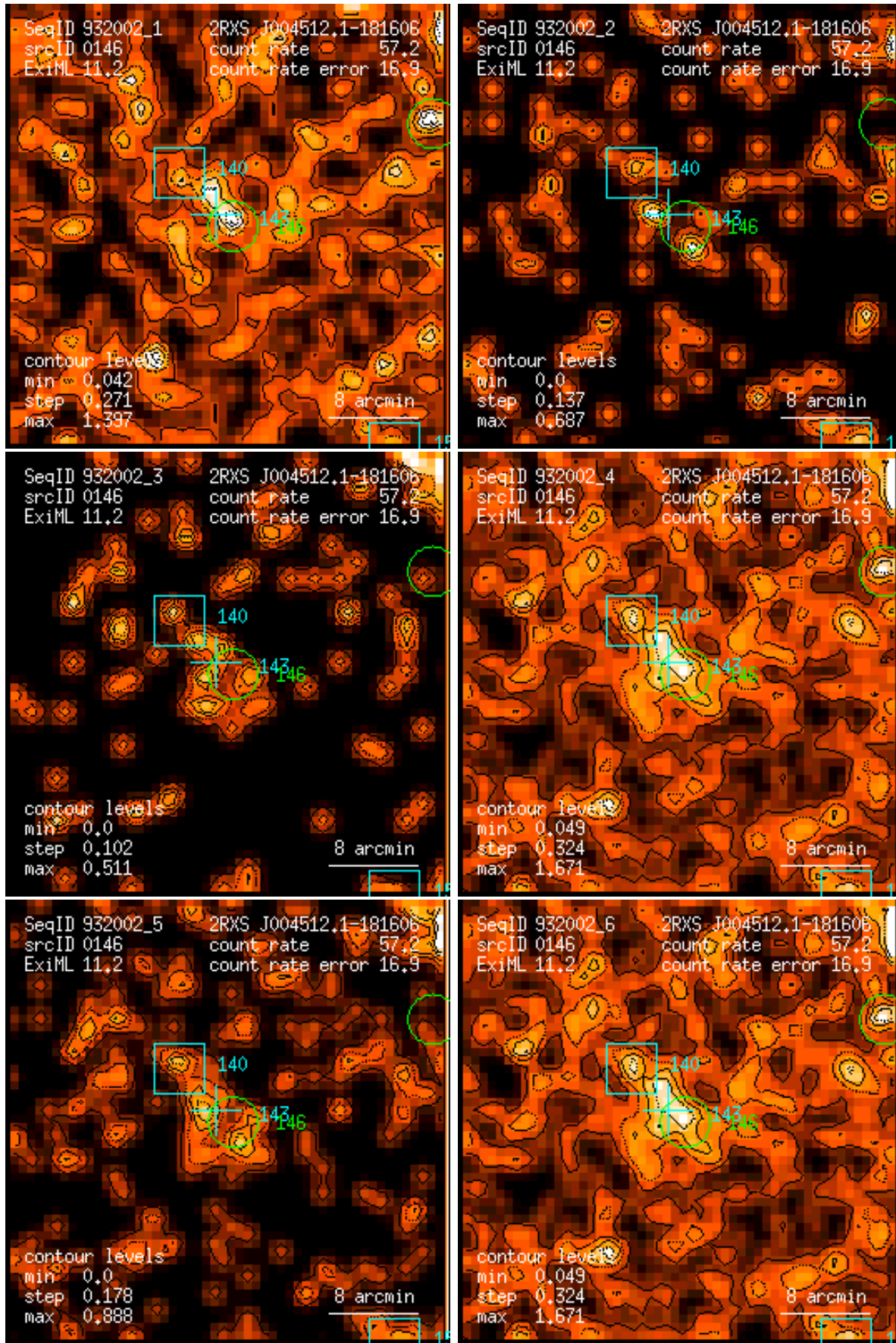
Figure 146: RASS 932002: detection 0146: band rate images, Gaussian filter: (1) PSPC channels 11 – 41, (2) 52 – 90, (3) 91 – 201, (4) 11 – 235, (5) 52 – 201, (6) 11 – 201. Broad band rates in counts/ks. Band rate contour levels in counts/ks/arcmin 2 .
