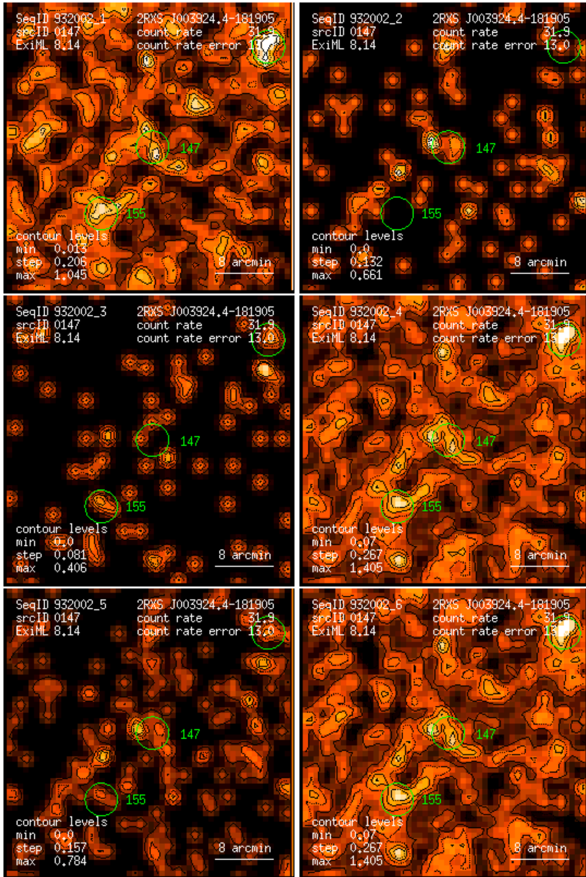
Figure 147: RASS 932002: detection 0147: band rate images, Gaussian filter: (1) PSPC channels 11 – 41, (2) 52 – 90, (3) 91 – 201, (4) 11 – 235, (5) 52 – 201, (6) 11 – 201. Broad band rates in counts/ks. Band rate contour levels in counts/ks/arcmin 2 .
