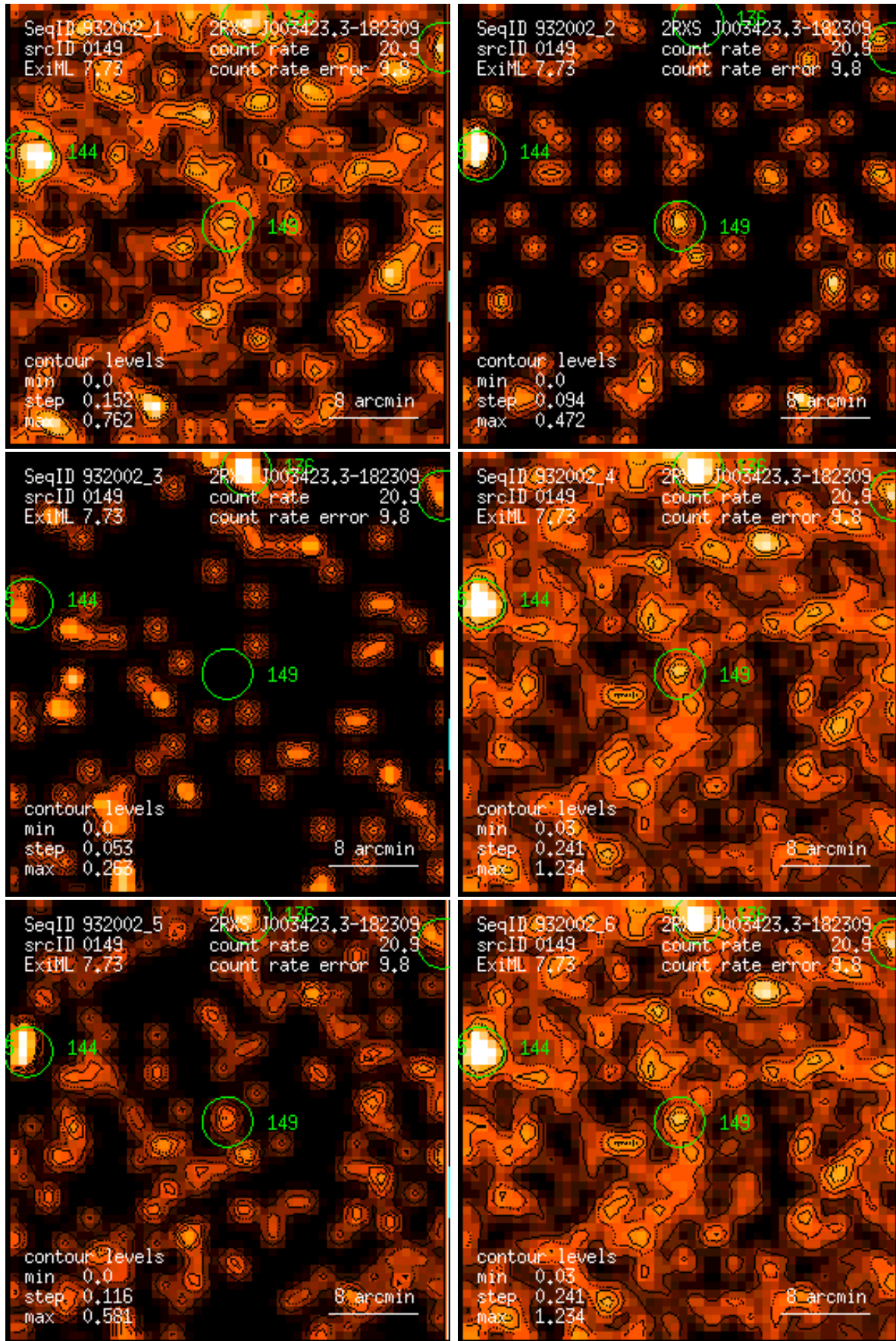
Figure 149: RASS 932002: detection 0149: band rate images, Gaussian filter: (1) PSPC channels 11 – 41, (2) 52 – 90, (3) 91 – 201, (4) 11 – 235, (5) 52 – 201, (6) 11 – 201. Broad band rates in counts/ks. Band rate contour levels in counts/ks/arcmin 2 .
