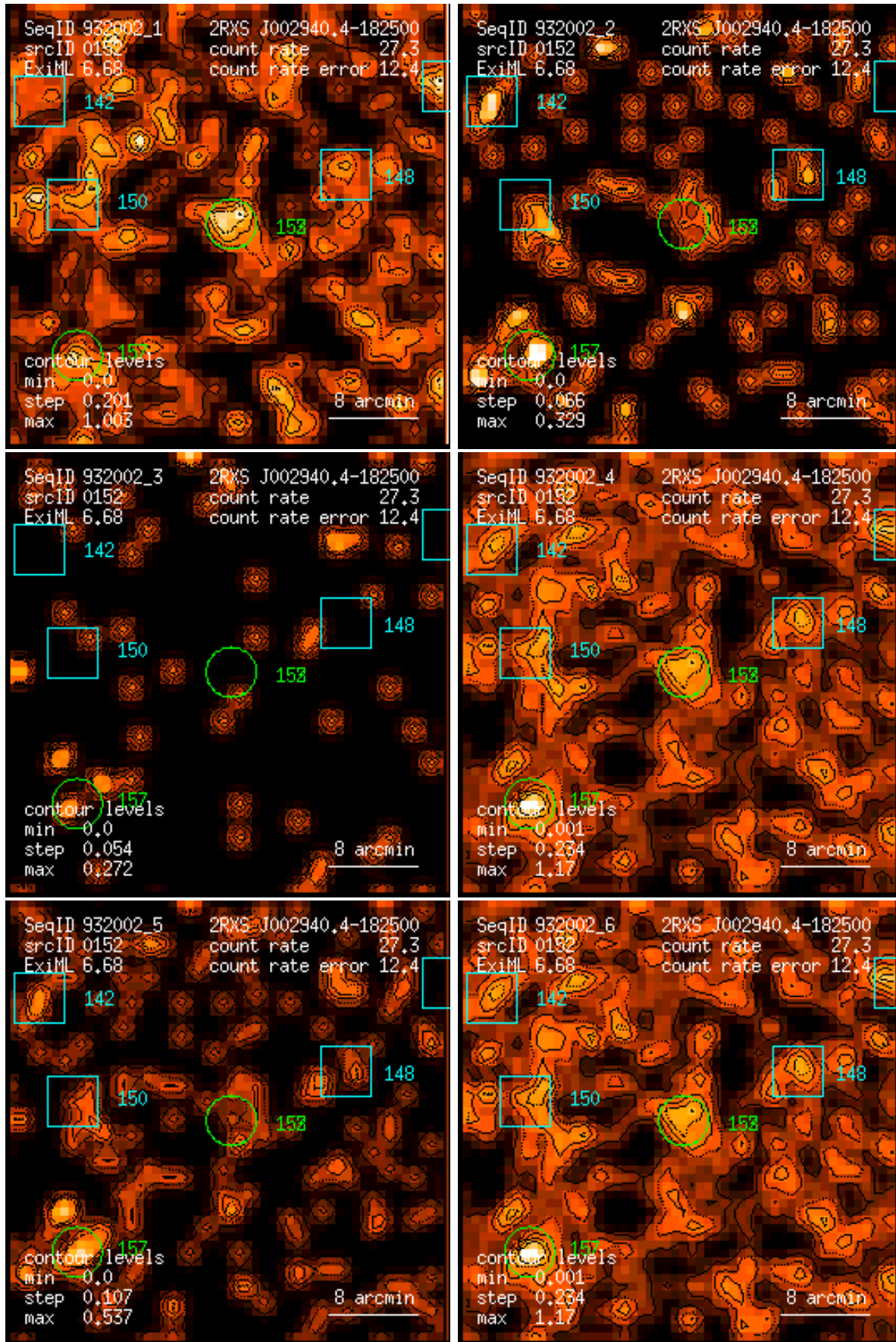
Figure 152: RASS 932002: detection 0152: band rate images, Gaussian filter: (1) PSPC channels 11 – 41, (2) 52 – 90, (3) 91 – 201, (4) 11 – 235, (5) 52 – 201, (6) 11 – 201. Broad band rates in counts/ks. Band rate contour levels in counts/ks/arcmin 2 .
