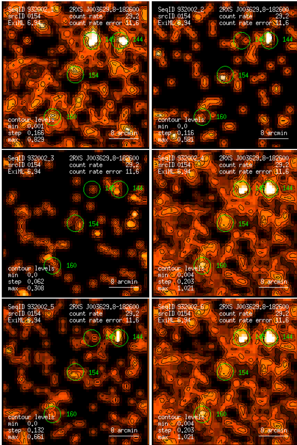
Figure 154: RASS 932002: detection 0154: band rate images, Gaussian filter: (1) PSPC channels 11 – 41, (2) 52 – 90, (3) 91 – 201, (4) 11 – 235, (5) 52 – 201, (6) 11 – 201. Broad band rates in counts/ks. Band rate contour levels in counts/ks/arcmin 2 .
