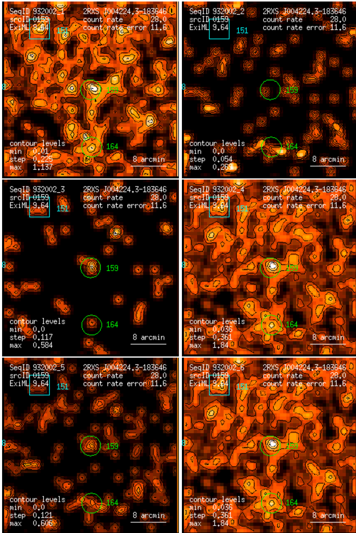
Figure 159: RASS 932002: detection 0159: band rate images, Gaussian filter: (1) PSPC channels 11 – 41, (2) 52 – 90, (3) 91 – 201, (4) 11 – 235, (5) 52 – 201, (6) 11 – 201. Broad band rates in counts/ks. Band rate contour levels in counts/ks/arcmin 2 .
