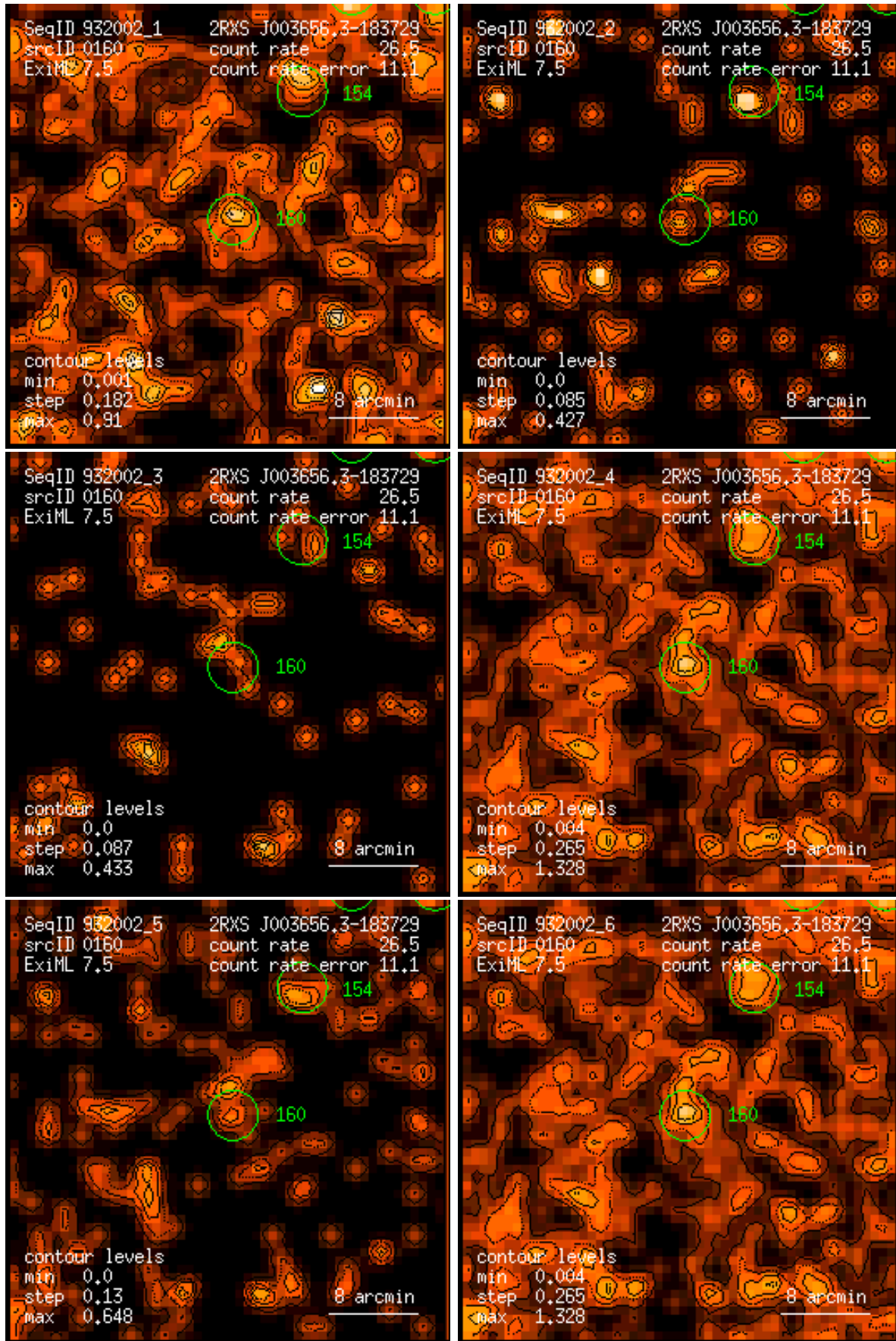
Figure 160: RASS 932002: detection 0160: band rate images, Gaussian filter: (1) PSPC channels 11 – 41, (2) 52 – 90, (3) 91 – 201, (4) 11 – 235, (5) 52 – 201, (6) 11 – 201. Broad band rates in counts/ks. Band rate contour levels in counts/ks/arcmin 2 .
