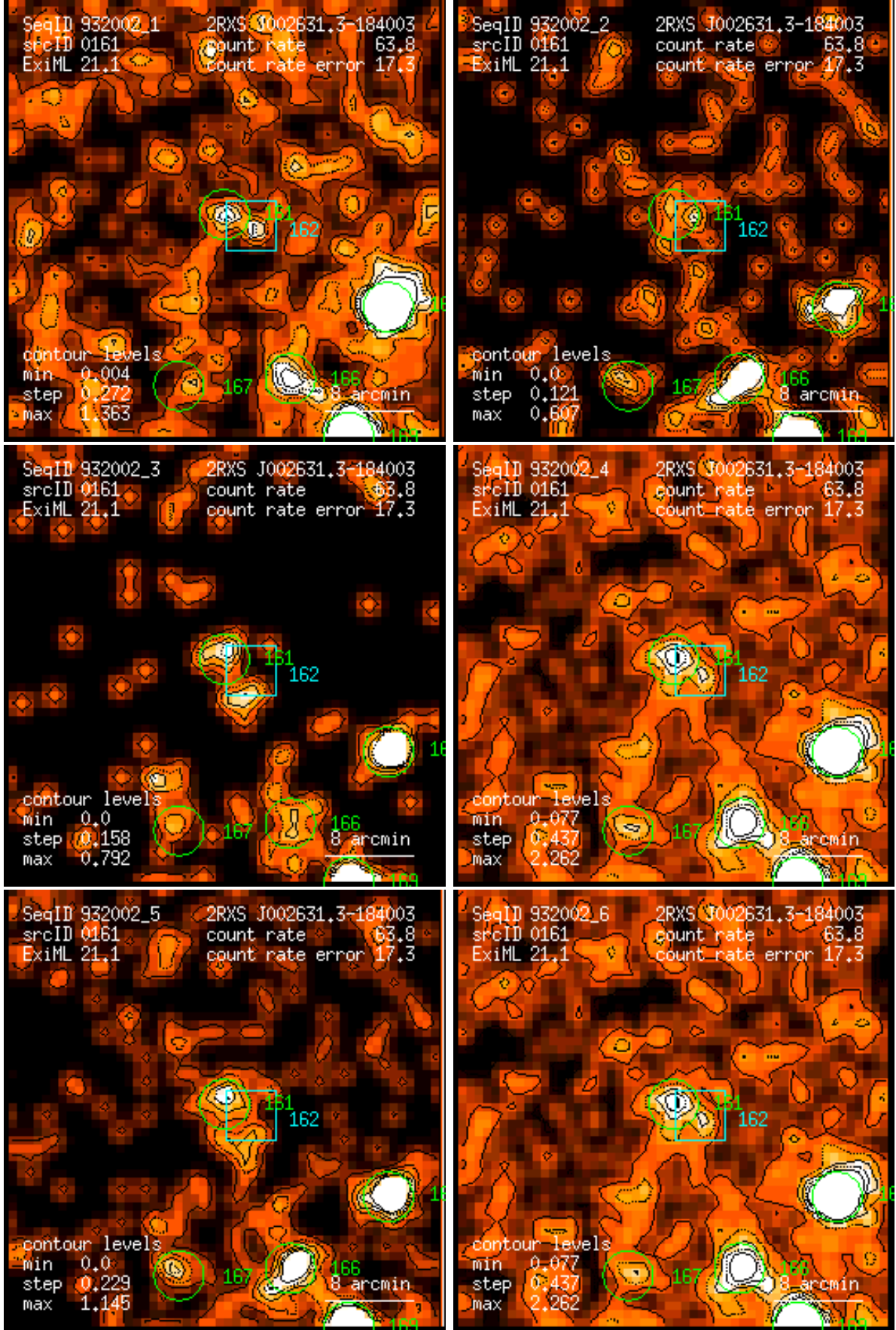
Figure 161: RASS 932002: detection 0161: band rate images, Gaussian filter: (1) PSPC channels 11 – 41, (2) 52 – 90, (3) 91 – 201, (4) 11 – 235, (5) 52 – 201, (6) 11 – 201. Broad band rates in counts/ks. Band rate contour levels in counts/ks/arcmin 2 .
