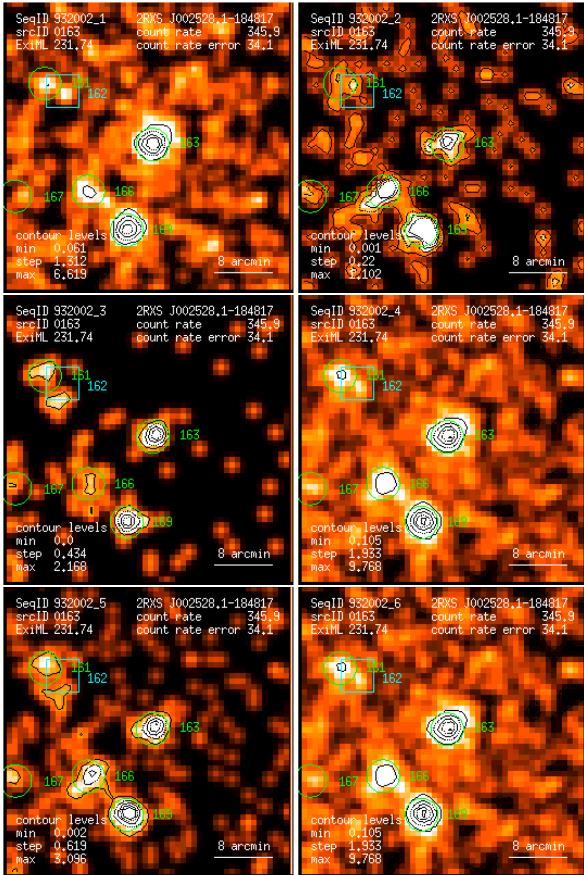
Figure 163: RASS 932002: detection 0163: band rate images, Gaussian filter: (1) PSPC channels 11 – 41, (2) 52 – 90, (3) 91 – 201, (4) 11 – 235, (5) 52 – 201, (6) 11 – 201. Broad band rates in counts/ks. Band rate contour levels in counts/ks/arcmin 2 .
