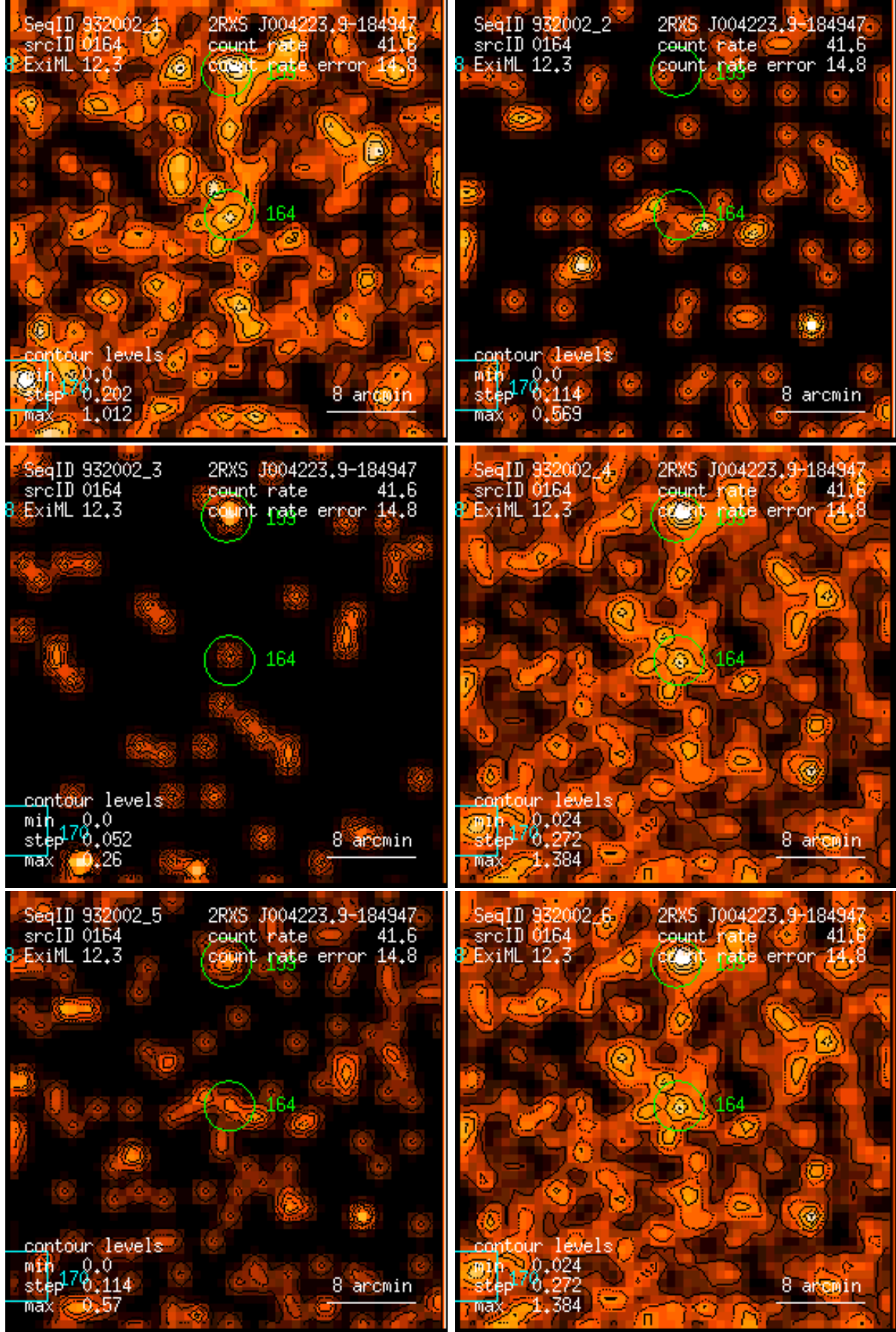
Figure 164: RASS 932002: detection 0164: band rate images, Gaussian filter: (1) PSPC channels 11 – 41, (2) 52 – 90, (3) 91 – 201, (4) 11 – 235, (5) 52 – 201, (6) 11 – 201. Broad band rates in counts/ks. Band rate contour levels in counts/ks/arcmin 2 .
