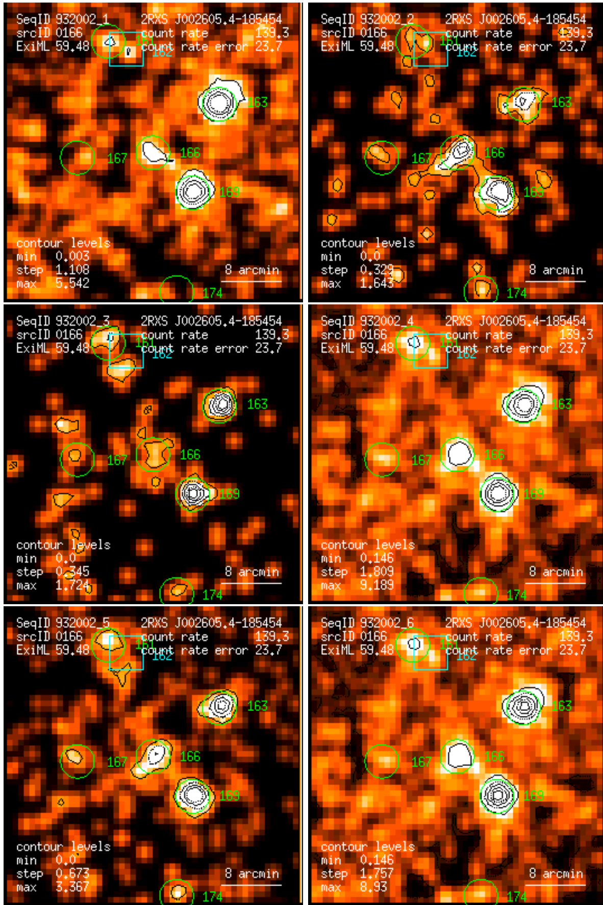
Figure 166: RASS 932002: detection 0166: band rate images, Gaussian filter: (1) PSPC channels 11 – 41, (2) 52 – 90, (3) 91 – 201, (4) 11 – 235, (5) 52 – 201, (6) 11 – 201. Broad band rates in counts/ks. Band rate contour levels in counts/ks/arcmin 2 .
