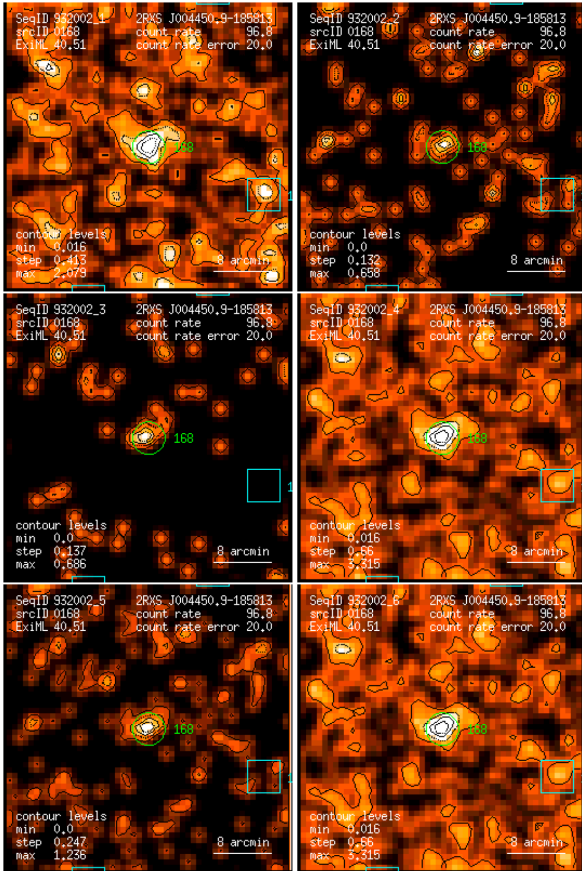
Figure 168: RASS 932002: detection 0168: band rate images, Gaussian filter: (1) PSPC channels 11 – 41, (2) 52 – 90, (3) 91 – 201, (4) 11 – 235, (5) 52 – 201, (6) 11 – 201. Broad band rates in counts/ks. Band rate contour levels in counts/ks/arcmin 2 .
