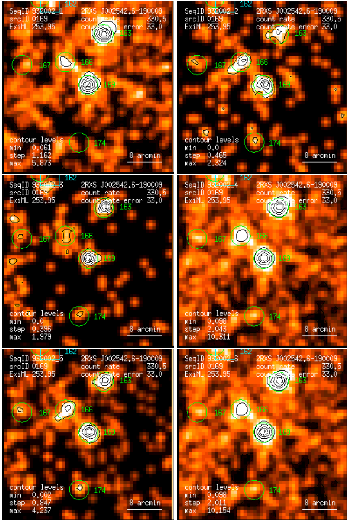
Figure 169: RASS 932002: detection 0169: band rate images, Gaussian filter: (1) PSPC channels 11 – 41, (2) 52 – 90, (3) 91 – 201, (4) 11 – 235, (5) 52 – 201, (6) 11 – 201. Broad band rates in counts/ks. Band rate contour levels in counts/ks/arcmin 2 .
