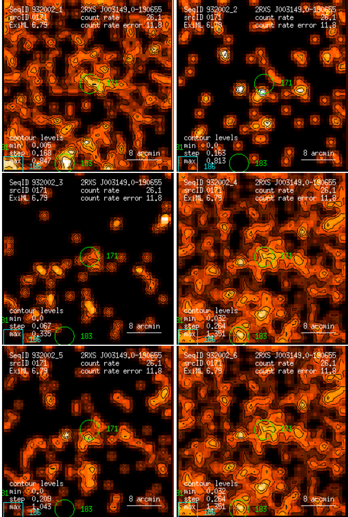
Figure 171: RASS 932002: detection 0171: band rate images, Gaussian filter: (1) PSPC channels 11 – 41, (2) 52 – 90, (3) 91 – 201, (4) 11 – 235, (5) 52 – 201, (6) 11 – 201. Broad band rates in counts/ks. Band rate contour levels in counts/ks/arcmin 2 .
