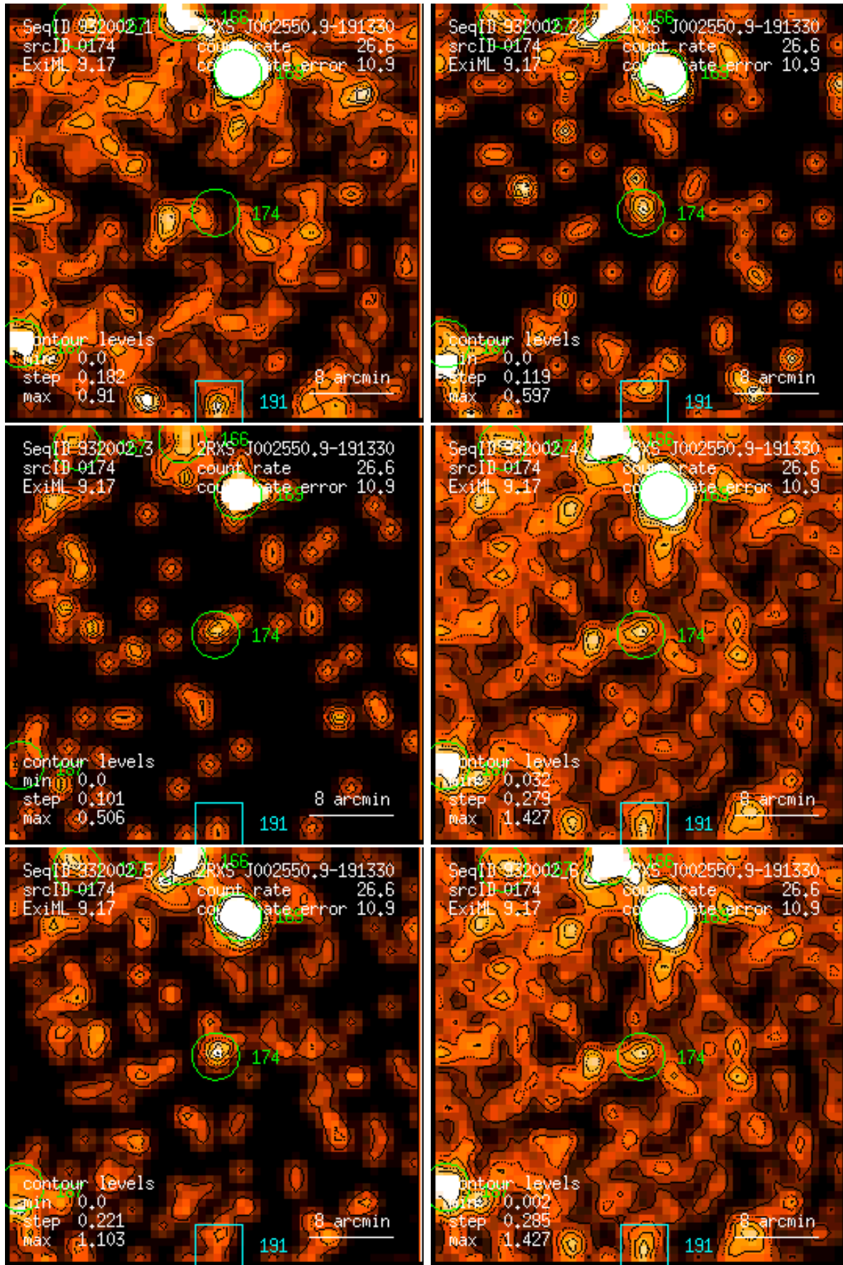
Figure 174: RASS 932002: detection 0174: band rate images, Gaussian filter: (1) PSPC channels 11 – 41, (2) 52 – 90, (3) 91 – 201, (4) 11 – 235, (5) 52 – 201, (6) 11 – 201. Broad band rates in counts/ks. Band rate contour levels in counts/ks/arcmin 2 .
