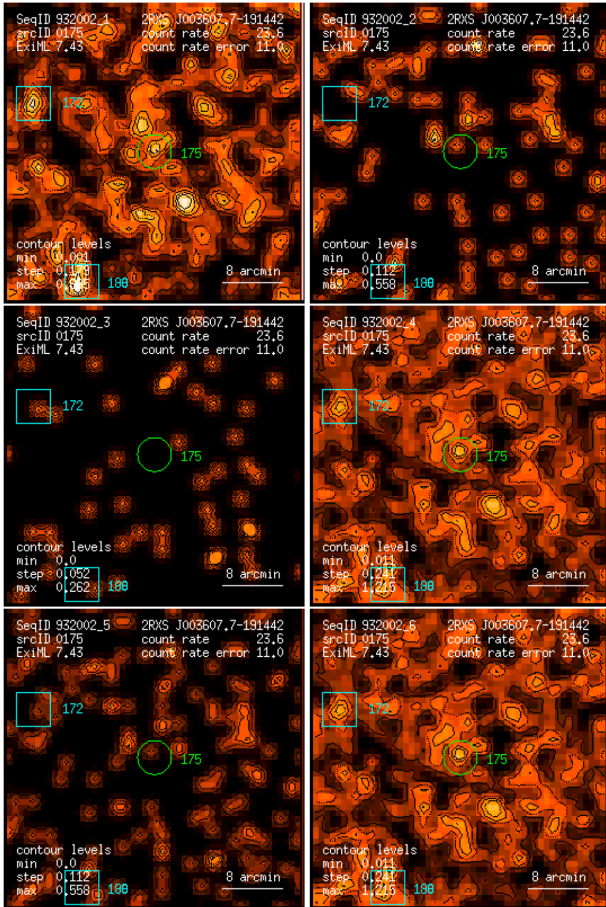
Figure 175: RASS 932002: detection 0175: band rate images, Gaussian filter: (1) PSPC channels 11 – 41, (2) 52 – 90, (3) 91 – 201, (4) 11 – 235, (5) 52 – 201, (6) 11 – 201. Broad band rates in counts/ks. Band rate contour levels in counts/ks/arcmin 2 .
